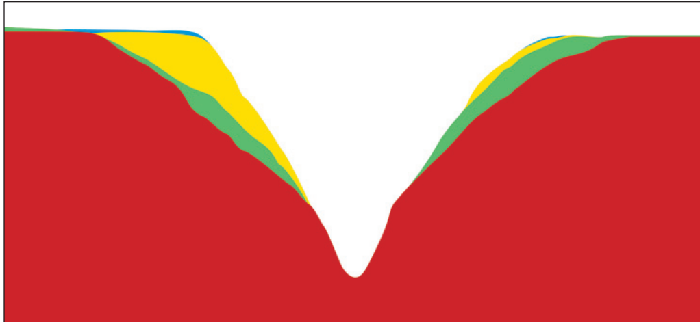
Figure 8. Model of soil cross-section showing extent of soil-loosening when strip-tilling is done when soil is wet (yellow) or dry (green). Red indicates soil that is not affected by the strip-tillage shank. Courtesy Randy Raper and Francisco Arriago, USDA ARS Soil Dynamics Laboratory, Auburn, Alabama, 2007.
