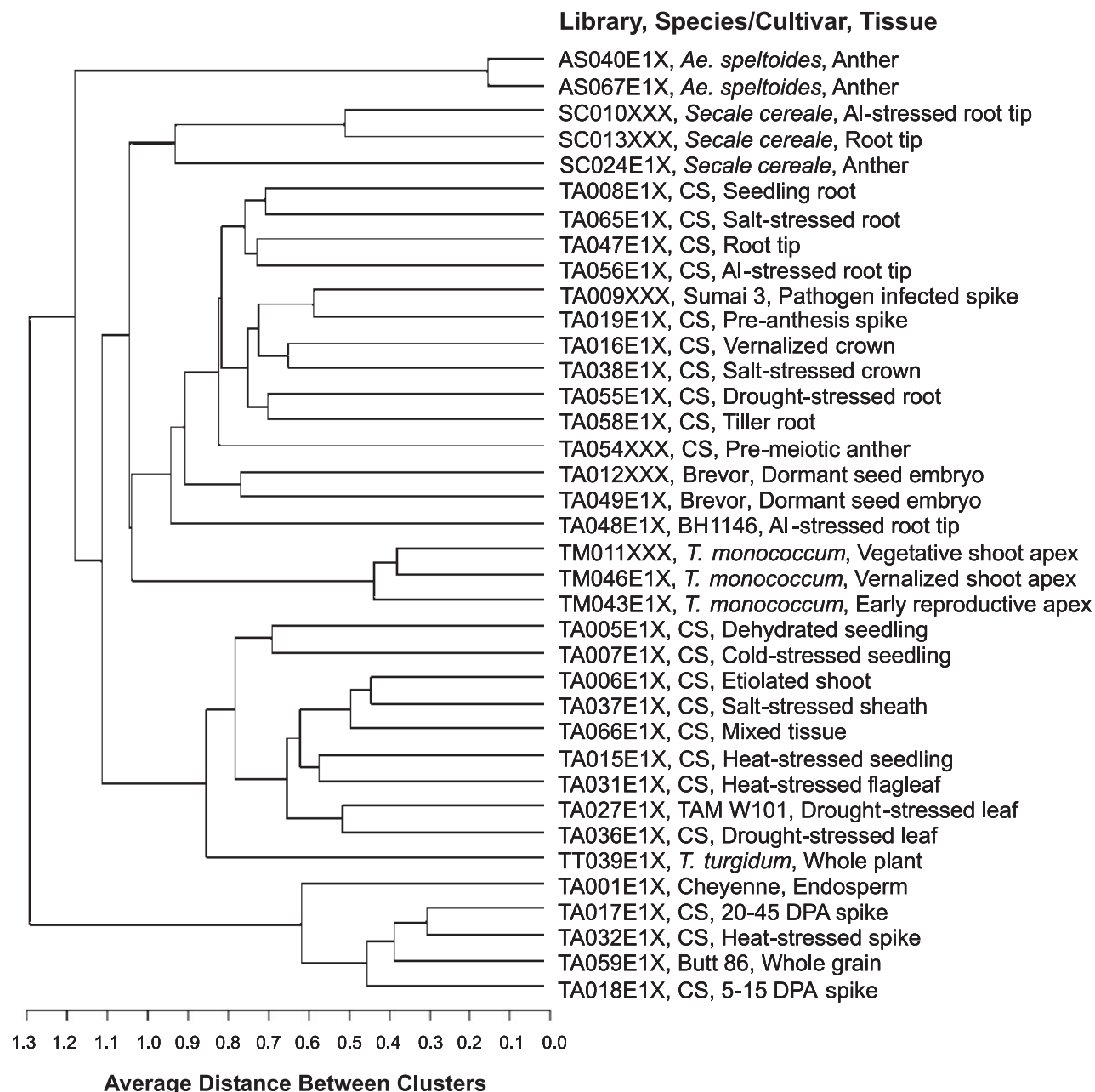
Fig. 2. The library dendrogram based on the cluster analysis data.
