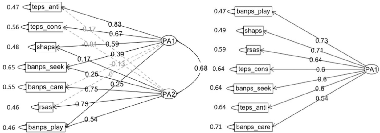
Figure 1. EFA factor loadings of Wave 8 data ( N = 173 ). On the left: PA1: Factor A from principal axis analysis; PA2: Factor B from principal axis analysis. RSAS: the Chapman Revised Social Anhedonia Scale; SHAPS: the Snaith-Hamilton Pleasure Scale; BANPS_Play, BANPS_Seek and BANPS_Care are the Play, Seek and Care subscales of the Brief Affective Neuroscience Personality Scale. TEPS_Anti and TEPS_Cons: the anticipatory and consummatory subscales of the Temporal Experience of Pleasure Scale. The grey dashed line indicates negative loadings from indicators. On the right, one factor was extracted and the indicators were sorted according to the loading size. No analytic constraints (e.g., fixed loadings) were applied.
