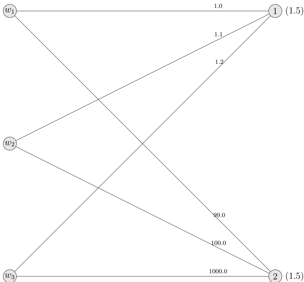
Figure B.2: An instance on which the optimal flow-guided algorithm outperforms the evaluation-guided algorithms EVALTPP and GREEDY in expectation. In addition, the flow-guided algorithm DISPATCH also outperforms the evaluation-guided algorithm GREEDY in expectation. To be precise, \text{OPT-FLOW}(W, J) > \text{EVAL-TPP}(W, J) > \text{DISPATCH}(W, J) > \text{GREEDY}(W, J) .
