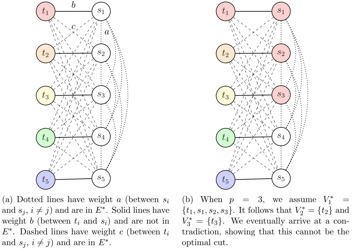
Figure 2.4: The construction used in theorem 2.2 when k = 5
