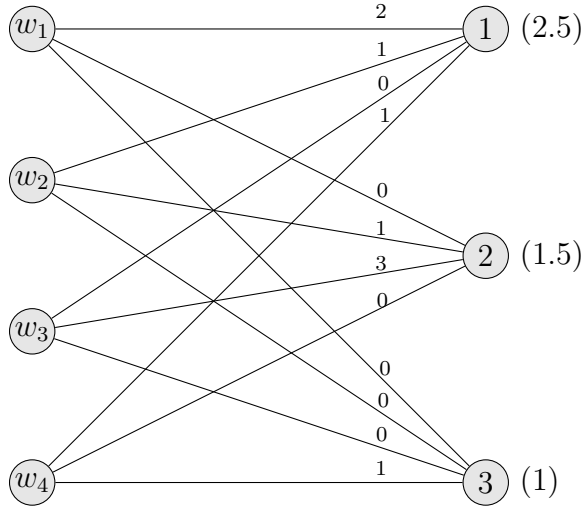
(a) An expectation graph with 4 workers and 3 job types. On one side, the workers. On the other side, the job types. In this example, p_1 = \frac{1}{2} and p_3 = \frac{1}{5} .
