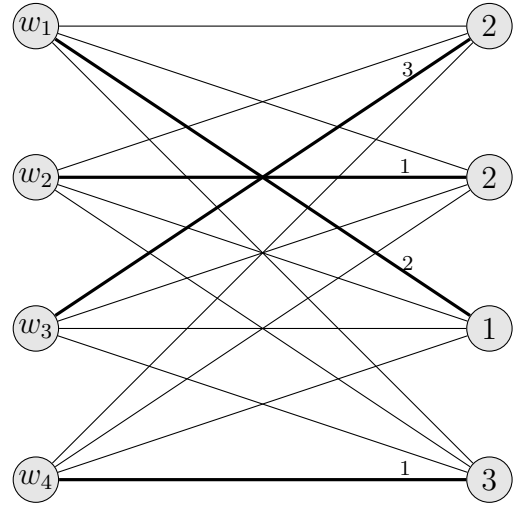
(b) A realization graph in which 2 workers of type 2 were sampled, then 1 worker of type 1, then 1 worker of type 3. The bold edges represent a greedy assignment of jobs to workers.
