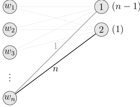
Figure 4.7: Instances in which the competitive ratio of a greedy algorithm tends to zero as the number of workers tends to infinity.
