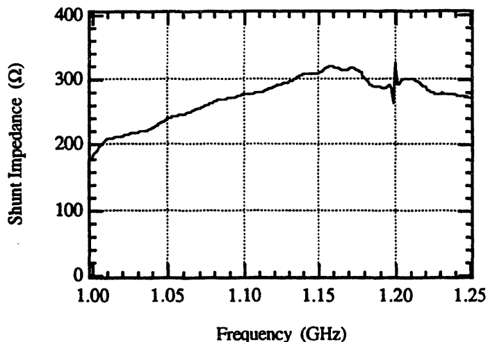
Figure 5. Longitudinal kicker shunt impedance
