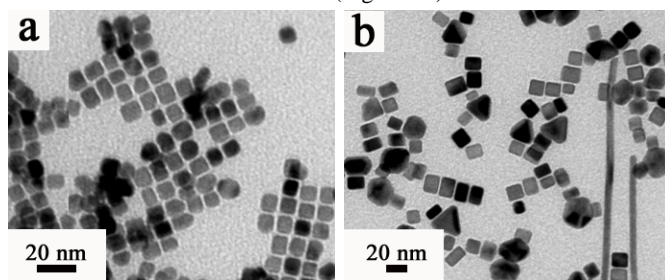
Figure 2. TEM images of (a) Pt and (b) Pd nanocubes.
