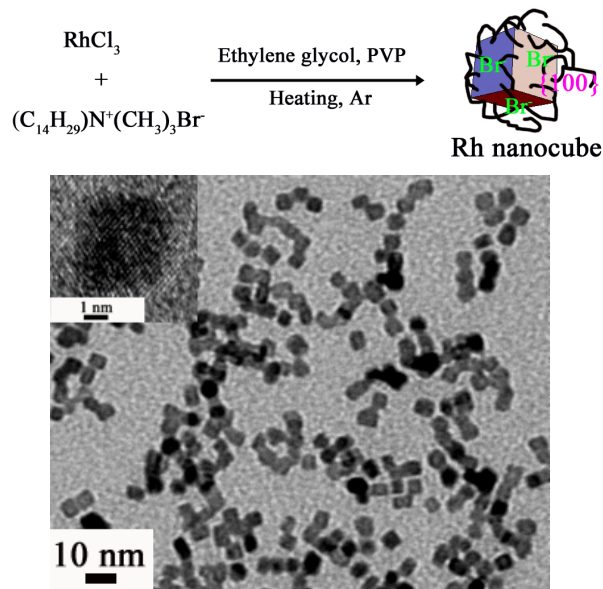
Figure 1. TEM and HRTEM (inset) images of Rh nanocubes.
