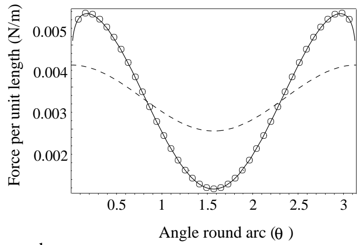
FIG. 2: Test configuration: a) shows a 1 \mu\text{m} artificially semi-circularly bowed, edge oriented, dislocation source, b) shows the magnitude of the self force as a function of angle round the bowed arc calculated using the numerical scheme (circles), the analytic solution (solid line), and using straight line tension approximation (dashed). The agreement between the exact result and the predictions of the computer model is excellent.
