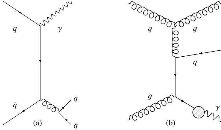
Figure 1: Examples of diagrams for \gamma + \text{jet} + \text{jet} production through (a) direct-photon and (b) fragmentation-photon processes.
