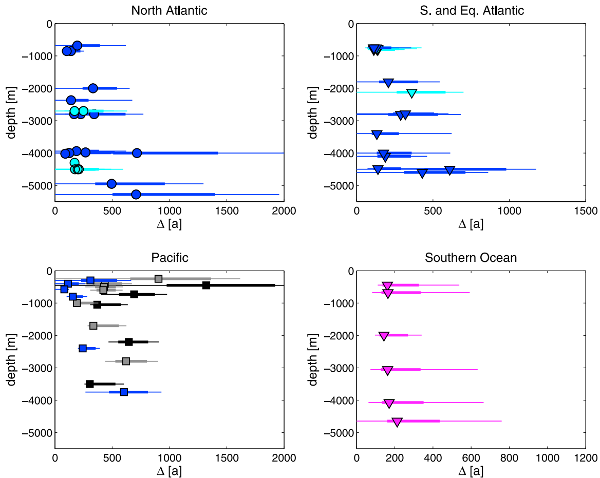
Figure 8. The TTD width, \Delta , using ^{39}\text{Ar} and the model prior. Error bars were estimated as discussed in Appendix B. Symbol shapes and colors identify the location of the ^{39}\text{Ar} measurements as in Figure 1. Note that different basins have different scales for \Delta .
