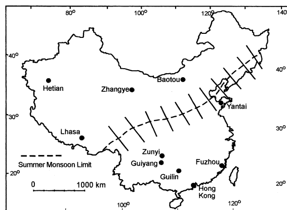
Fig. 2. Map indicating the locations of 10 sites in the IAEA/GNIP database selected for use in this study. The cross-hatched area denotes the approximate northern limit of the summer monsoon.
