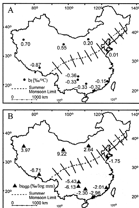
Fig. 9. Maps showing linear regression slopes (A) \beta_T and (B) \beta_{\log P} for the 10 IAEA/GNIP sites. Comparison with Fig. 7 suggests that with a simple linear model, the dependence of \delta^{18}\text{O}_p on temperature may be overestimated while dependence on precipitation amount may be underestimated, especially for sites in Southern China.
