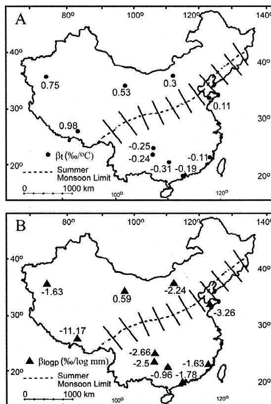
Fig. 7. Maps showing partial regression slopes (A) \beta_t ( \text{‰}/^\circ\text{C} ) and (B) \beta_{\log P} ( \text{‰}/\log \text{mm} ) for the 10 IAEA/GNIP sites.
