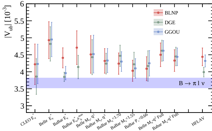
Fig. 6.1 Measurements of inclusive |V_{ub}| and their averages based on BLNP, DGE and GGOU calculations. The HFLAV average of |V_{ub}| results from B \rightarrow \pi l \nu_\ell decay is also reported for comparison.
