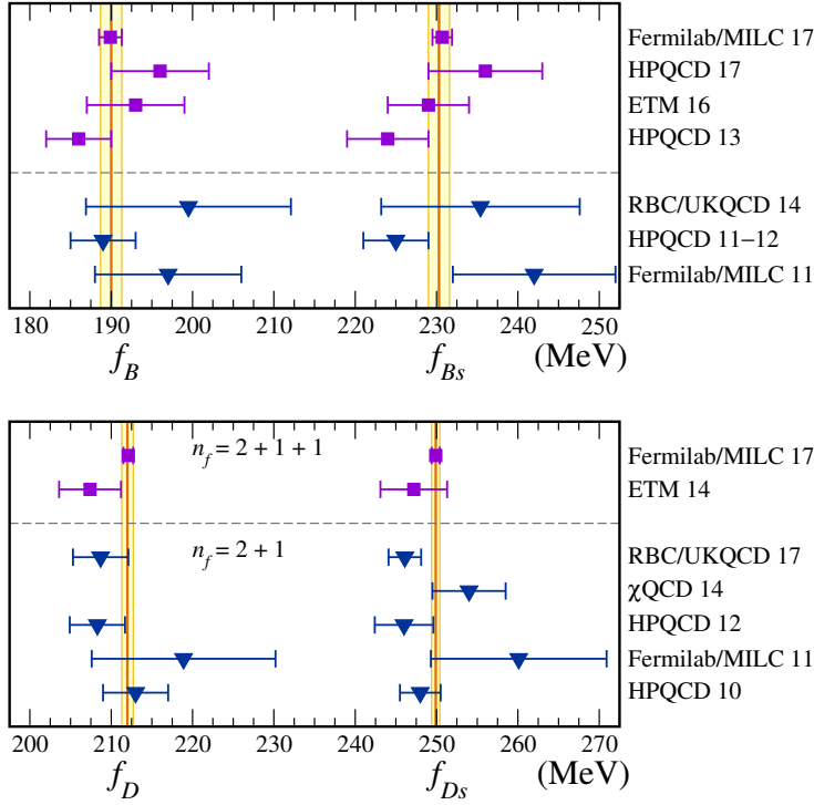
Fig. 4.2 Comparison of results for the B_{(s)} -meson (top) and the D_{(s)} -meson (bottom) decay constants. Squares denote lattice-QCD calculations with 2+1+1 flavors of sea quark [23,304, 27,305,306]; triangles denote lattice-QCD calculations with 2+1 flavors of sea quark [285,307, 264,308,309,310,311,20]. The vertical bands show the FLAG 2019 average for 2+1+1 sea flavors [3].
