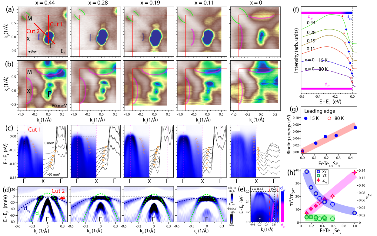
FIG. 3: Fermi surface evolution with Se ratio x . (a) Measured Fermi surfaces for different Se ratio x at 15 K except that for x = 0 , which is measured at 80 K above its magnetic transition. (b) Simultaneously measured constant energy contours at -60 meV showing no change. (c) Corresponding band dispersions and momentum distribution curves (MDCs) along the \Gamma -X- \Gamma direction. The markers are peaks fitted from MDCs. The MDCs are for binding energies from 0 meV to 60 meV. (d) Band dispersions (second derivative) measured with 22 eV photons at 10 K along the \Gamma -M direction around the Brillouin zone center for different x . Parabolic fittings of the d_{yz} and d_{xy} hole bands are overlaid. The red arrow in left-most panel of (d) points at the hybridization of d_{yz} and d_{xy} orbitals. (e) Band dispersion of \text{FeTe}_{0.56}\text{Se}_{0.44} at 15 K along the \Gamma -X- \Gamma direction. (f) Integrated energy distribution curve (EDC) around X of \text{FeTe}_{1-x}\text{Se}_x with the integral range marked by the red dashed lines in (e). The energy positions where the integrated EDCs show a maximum curvature are marked by the red bars. The leading edge marked by the blue and red circles represents the energy position where the EDC intensity is half of where at the maximum curvature. (g) Leading edge determined in (f) versus Se content of \text{FeTe}_{1-x}\text{Se}_x . (h) Extracted band enhancement factor m^*/m_{\text{DFT}} for d_{yz} and d_{xy} plotted as a function of x represented by circles. The shaded lines are guides to the eyes. Diamond markers show the inverse of the d_{xy} mass enhancement where the shaded pink line is a linear fit. The empty markers are reproduced from Liu et al. [60].
