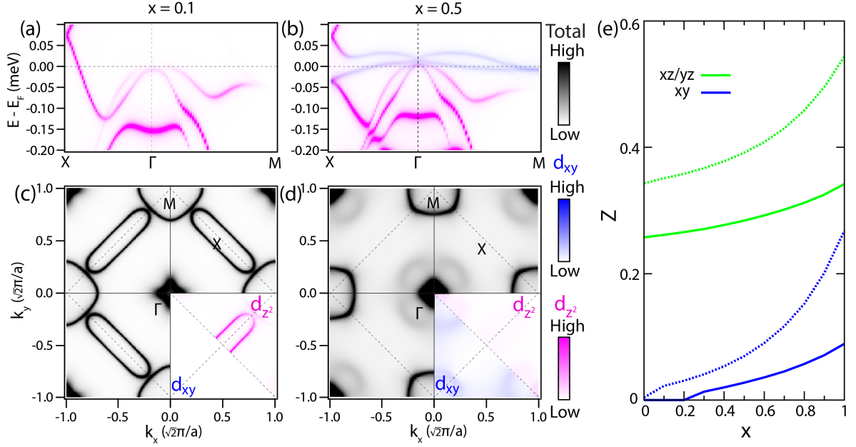
FIG. 4: Theoretical calculations of \text{FeTe}_{1-x}\text{Se}_x . (a)-(b) Calculated band structure projected onto different orbitals for the orbital-selective Mott phase \text{FeTe}_{0.9}\text{Se}_{0.1} and the strongly correlated metallic phase in \text{FeTe}_{0.5}\text{Se}_{0.5} , respectively. The magenta intensity indicates d_{z^2} orbital character, whereas blue intensity the d_{xy} orbital. (c) Calculated Fermi surface for \text{FeTe}_{0.9}\text{Se}_{0.1} , where the lower right quadrant shows the d_{z^2} and d_{xy} intensity respectively. (d) Same as (c) but for \text{FeTe}_{0.5}\text{Se}_{0.5} . (e) Orbital-resolved coherence factor Z as a function of x . The solid line represents U = 3 eV and dashed line represents U = 2.65 eV. U denotes the intraorbital Coulomb repulsion.
