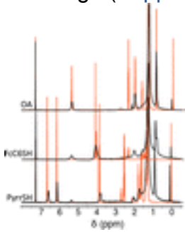
Figure 3. ^1\text{H} NMR spectra of the bound (black) and free (red) oleic acid (OA), FcC6SH, and PyrSH. Distinctive peaks at 5.35 ppm (OA), 4.05 ppm (FcC6SH), and 6.15 ppm (AlkylSH) were used to quantify the number of ligands bound per nanocrystal. FcC3SH appears also at 4.05 ppm, but is broader due to it being closer in distance to the nanocrystal surface ( Supporting Information ).
