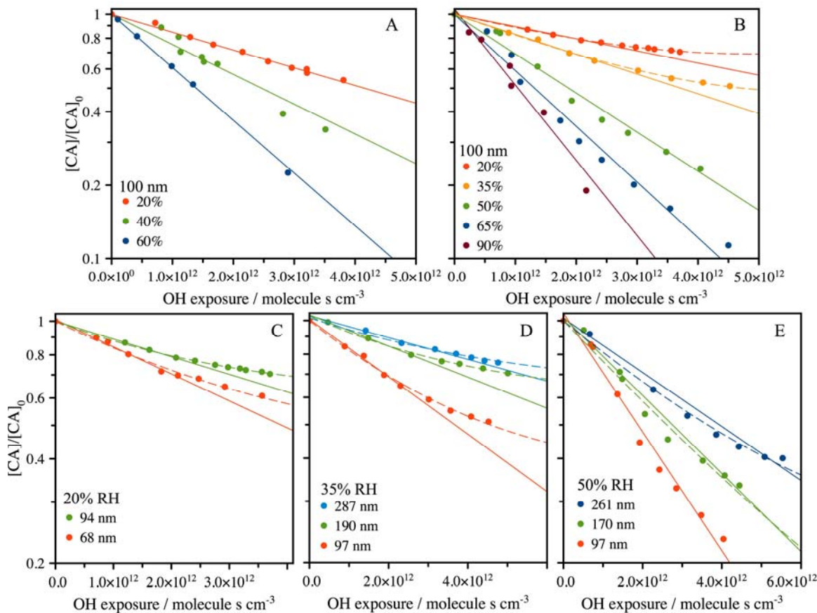
Figure 2: Reactive decay of 100 nm size-selected CA aerosol (inferred from the intensity of the peak at m/z 191.02) vs. RH (20% to 90%,) using: (A) the DART heater to probe the surface of the aerosol during ionisation; and (B) an oven to fully vaporise the aerosol prior to ionisation. Kinetic decay plots for fully vaporised size-selected CA aerosol at 20% RH (C), 35% RH (D) and 50% RH (E). A pure exponential decay function is shown by the solid lines, with low RH data fit only at early exposure. A fit to the accessible volume model is shown by the dashed lines, with best fit k and L tabulated in Table 1.
