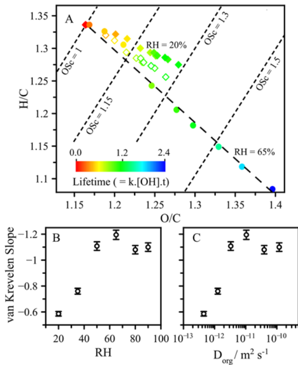
Figure 5: (A) van Krevelen diagram showing oxidation at RH = 65% (solid circles), RH = 20% (solid diamonds). RH = 20% with the contribution of the functionalised alcohol removed (open diamonds), as described in the text. Slope of the product data in van Krevelen space as a function of: (B) and (C) diffusion coefficient.
