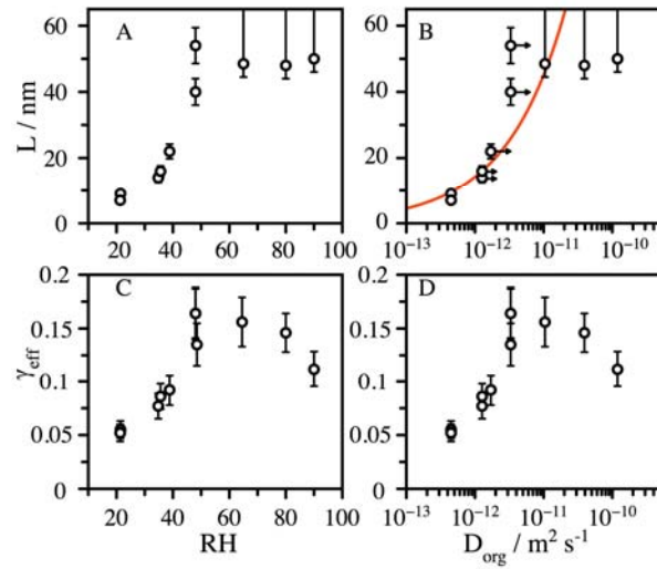
Figure 3: Accessible reaction depth, L , inferred from the reactive decay kinetics of CA with OH as a function of: (A) the RH, and (B) the diffusion constant estimated using the Stokes-Einstein relationship. Horizontal arrows show the change in D_{\text{org}} when corrected for water uptake during the reaction. The red line shows the square-root dependence of L on D_{\text{org}} . Effective uptake coefficient, \gamma_{\text{eff}} , as a function of: (C) the RH, and (D) the diffusion constant.
