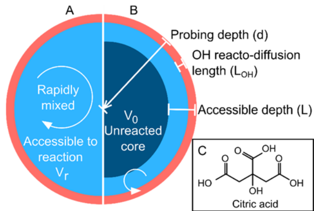
Figure 1: Schematic of (A) a well-mixed droplet; and (B) a droplet with a limited accessible reaction volume defined by depth, L . (C) Molecular structure of citric acid.
