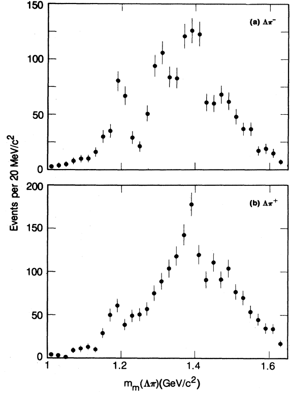
FIG. 27. (a) Missing mass opposite \Delta\pi^- events, where \Xi^- \rightarrow \Delta\pi^- events have been excluded and (b) missing mass opposite \Delta\pi^+ events. The peak near 1.32 \text{GeV}/c^2 in (a) is from feedthrough of the decay \psi \rightarrow \Xi^-\bar{\Xi}^+ , the peaks near 1.38 \text{GeV}/c^2 in (a) and (b) are due to the decays \psi \rightarrow \Sigma(1385)\bar{\Sigma}(1385) , and the peaks near 1.19 \text{GeV}/c^2 in (a) and (b) are due to the decays \psi \rightarrow \Lambda\Sigma\pi .
