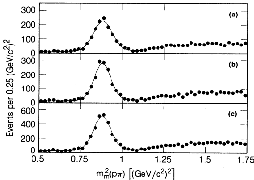
FIG. 23. m_m^2 against N\pi system, (a) p\pi^- , (b) \bar{p}\pi^+ , and (c) both charge modes. The peaks near m_m^2 = 0.88 \text{ (GeV}/c^2)^2 are from the decays \psi \rightarrow \bar{p}\pi^+ n . Solid curves are described in text.
