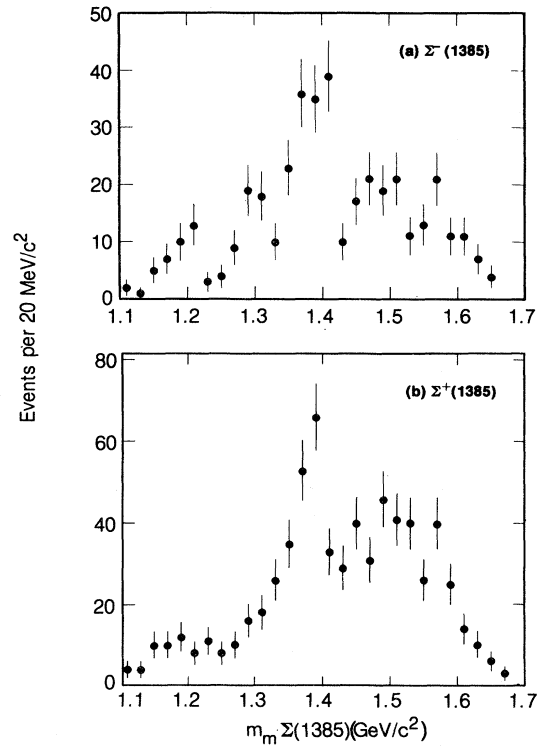
FIG. 14. (a) Missing mass against \Sigma^-(1385) and (b) missing mass against \Sigma^+(1385) . The peaks near 1.38 \text{GeV}/c^2 in both (a) and (b) are due to the decays \psi \rightarrow \Sigma(1385)\bar{\Sigma}(1385) , while the peaks near 1.19 \text{GeV}/c^2 in both (a) and (b) are primarily due to reactions (33) and (35). Here, we denote as \Sigma(1385) a \Lambda\pi system in the mass region defined in the text.
