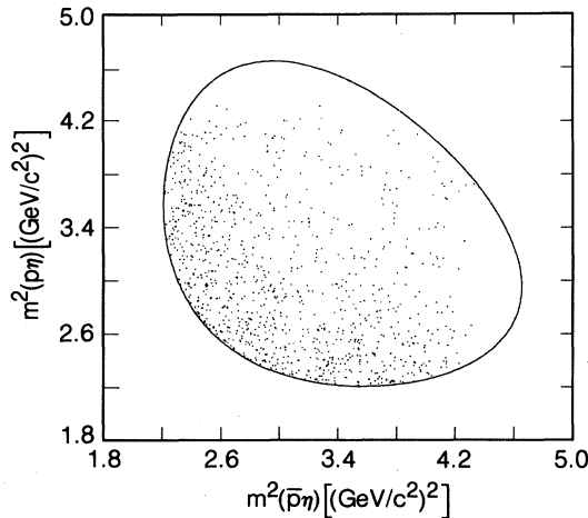
FIG. 29. Dalitz plot for \psi \rightarrow p\bar{p}\eta . The events in this plot have been kinematically constrained to the event hypothesis.
