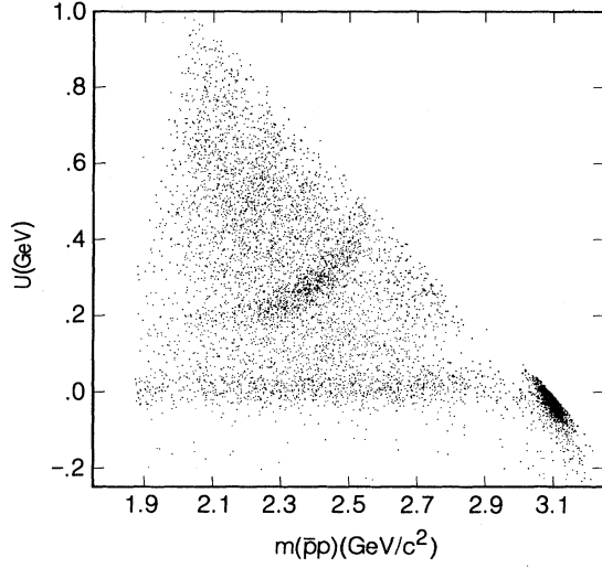
FIG. 16. Scatterplot of p\bar{p} mass versus U , in all p\bar{p} pairs. The band in the vicinity of U=0.3 GeV is due to the decay \psi \rightarrow p\bar{p}\eta , while the band near U=0 GeV is due to the decays \psi \rightarrow p\bar{p}\gamma(\pi^0) . The dark region near m(p\bar{p})=3.1 GeV/ c^2 is from the decay \psi \rightarrow p\bar{p} .
