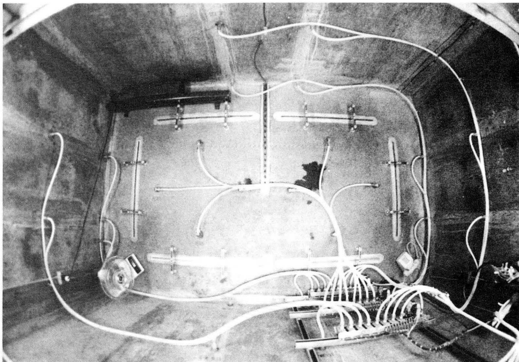
Bird's-eye view of instrumentation in one of the radon group's "small structures," essentially an enclosed basement in the Santa Cruz mountains.
