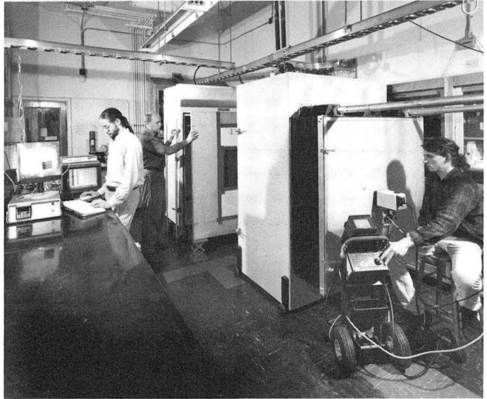
Brent Griffith, left, and Radim Jasek prepare a sample window for testing in the infrared thermography facility. Paul Donohoe, far right, adjusts the infrared camera. The structure attached to the bellows is the newly built room temperature chamber that maintains environmental conditions as constant as those in the refrigerated chamber to its left.
