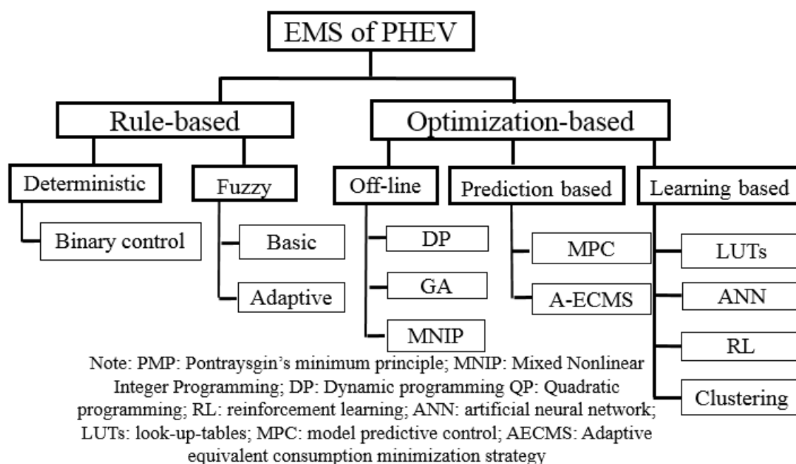
Fig.2. Basic classification of EMS for PHEV.
