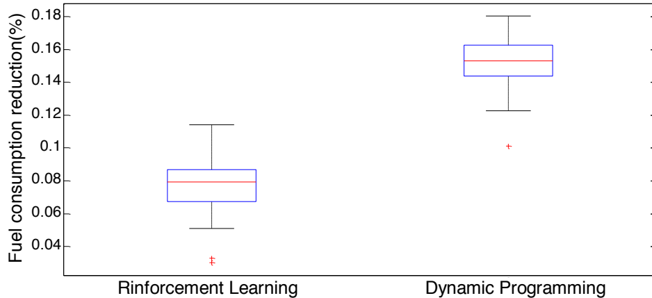
Fig. 26. Fuel consumption reduction compared to binary control.
