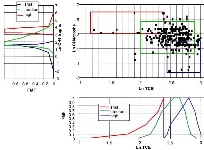
Figure 4. Fuzzy graph of the relationship between logarithms of TCE and methanotrophs concentrations for wells 1C-3C and 5C-10C and corresponding FMFs plotted parallel to the axes.
