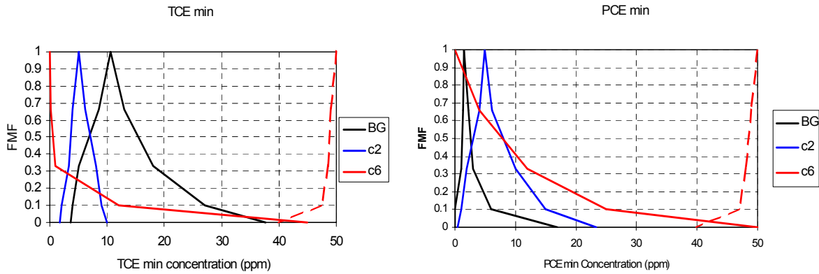
Figure 3. Fuzzy membership functions for TCE and PCE mineralization, which compare the performance of air stripping (Campaign 2 - c2) and bioremediation (Campaign 6 - c6) with background conditions (BG)
