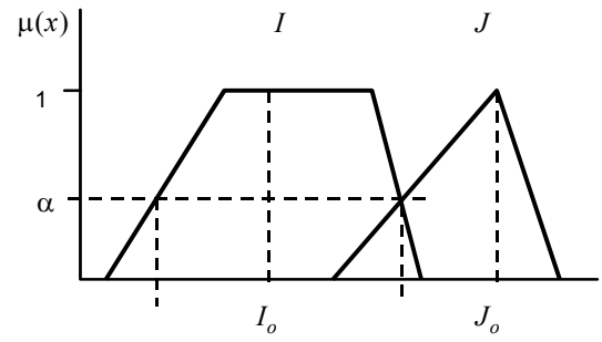
Figure 2. Comparison of two fuzzy numbers: J > I for \mu(x) > \alpha ( I_o and J_o are crisp numbers)
