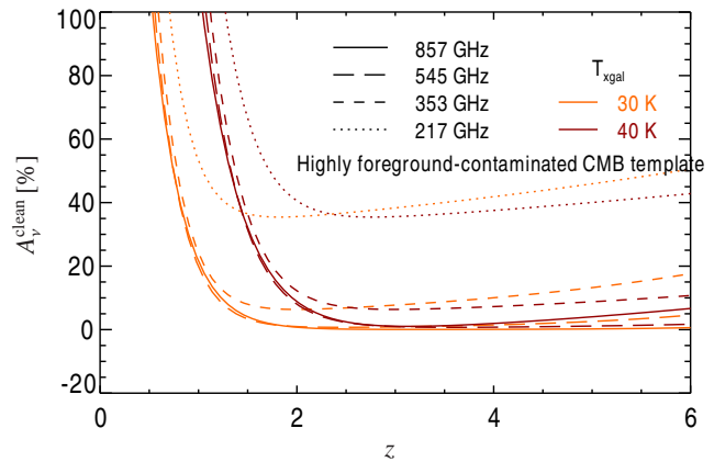
Fig. 5. Relative attenuation coefficient A_{\nu}^{\text{clean}} due to the cleaning process, as a function of redshift for each Planck -HFI band. This is computed for two input SEDs modelled by a modified blackbody ( T_{\text{xgal}} = 30 K and 40 K, with \beta_{\text{xgal}} = 1.5 ) embedded in foreground emission equally balanced between CIB and Galactic cirrus. It is shown for two extreme cases of the CMB template quality, i.e., ideal (upper panel) or highly contaminated by extragalactic foregrounds at high \ell (lower panel).
