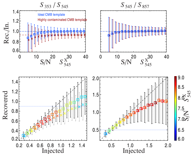
Fig. 10. Colour-colour ratio recovery. Left: S_{353}/S_{545} . Right: S_{545}/S_{857} . Top: ratio of recovered over injected colour-colour ratio (Rec./In.) as a function of the 545 GHz excess S/N. This is shown for two choices of the CMB template, i.e., ideal (blue squares) or highly contaminated by extragalactic foregrounds (red crosses). Bottom: recovered versus injected colour-colour ratio per bin of input colour-colour ratio. Again, two cases are shown depending on the quality of the CMB template, ideal (squares) or highly contaminated (crosses). The colour scale provides the average S/N of the 545 GHz excess inside each bin of input colour-colour ratio. The blue dotted lines show S_{353}/S_{545} < 0.9 and S_{545}/S_{857} > 0.5 , which are the colour criteria adopted for source selection.
