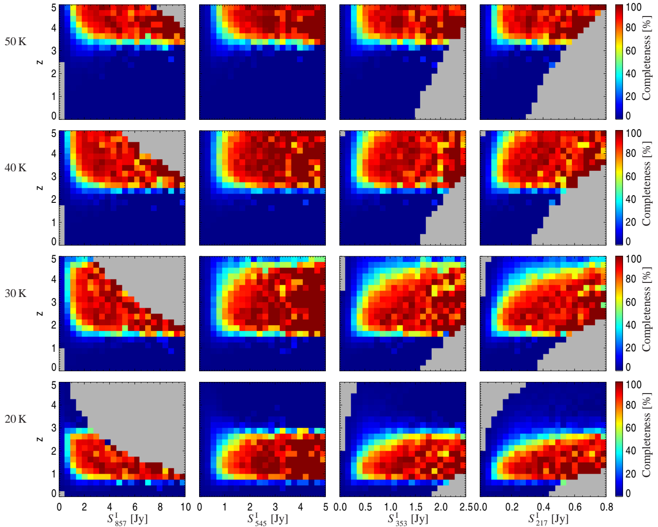
Fig. 11. Completeness as a function of redshift and flux density at 857, 545, 353, and 217 GHz (from left to right) and for each category of injected sources with dust temperatures of 20, 30, 40, and 50 K, from top to bottom, respectively. Grey regions are domains without simulated data for these flux densities and redshifts.
