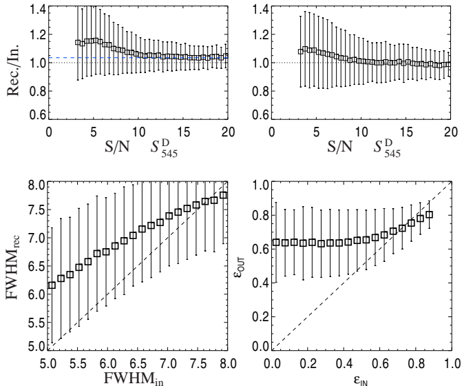
Fig. 8. FWHM and ellipticity recovery. Left: FWHM. Right: ellipticity. Top: ratio of recovered over injected FWHMs and ellipticities (Rec./In.) as a function of the S/N of detection on the 545 GHz cleaned map. Bottom: recovered versus injected FWHMs and ellipticities. The dashed line gives the 1:1 relation.
