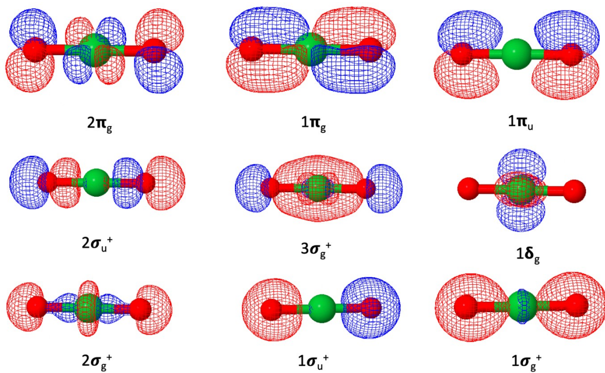
Figure 3. Valence molecular orbitals of \text{NiO}_2 originating from the Ni 4s and 3d orbitals and the O 2s and 2p orbitals.
