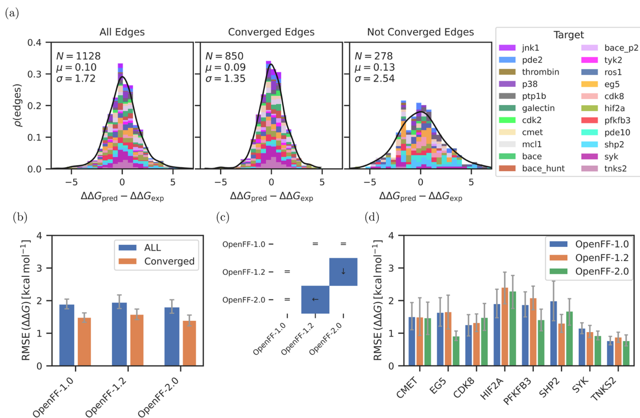
Figure 5. Comparison of the three force fields OpenFF-1.0, OpenFF-1.2, and OpenFF-2.0 based on the \Delta\Delta G values. Panel (a) shows the absolute error distributions between experimental and calculated \Delta\Delta G using OpenFF-2.0 for three sets of edges. First set in the left subpanel contains all edges, the second set in the center contains only converged edges, and the third set in the right contains the not converged edges (which is the difference set between the first and second set). See the Methods Section for more details about the convergence criteria. Different colors denote the different targets and the black line is a normal distribution fitted to the data. Text in the panel lists the number of edges N , the center \mu , and the standard deviation \sigma of the normal distribution. Panel (b) shows the RMSE across all edges of 8 targets for the three force fields of the OpenFF family. Blue bars correspond to all edges and the orange bars only to the converged ones. Panel (c) illustrates significant differences between the force field sets shown in panel (b). White matrix element with an equal sign (“=”) means that the differences between the two force fields are statistically insignificant. Blue matrix element denotes a significant difference considering a 95% confidence interval. Arrow in a blue matrix element points at the force field, which has the lower error. Panel (d) shows the RMSE of the \Delta\Delta G values per target for the three force fields OpenFF-1.0, OpenFF-1.2, and OpenFF-2.0. Lower and upper bound of the 95% confidence interval are given as error bars. All values are in \text{kcal mol}^{-1} .
