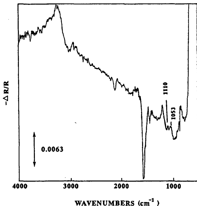
Figure 7. FTIR spectrum of the surface in Fig. 6 after raising the temperature to 160 K.
