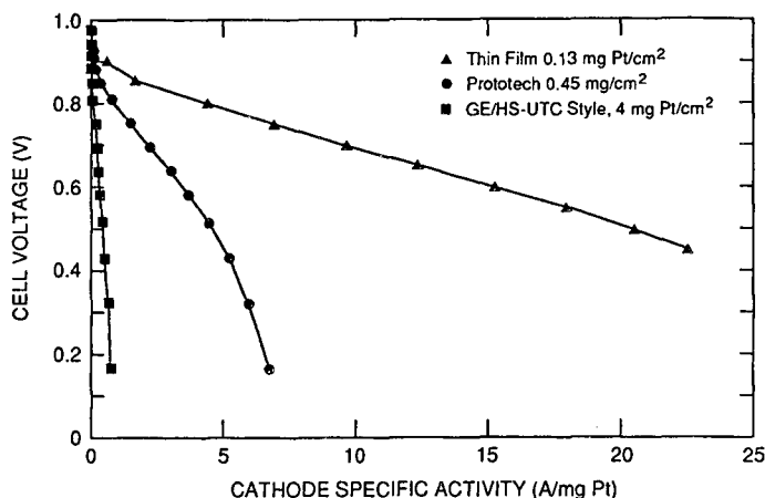
Figure 14. Comparison of specific Pt catalyst activities in PEFCs with three different types of Pt catalyst layers.
