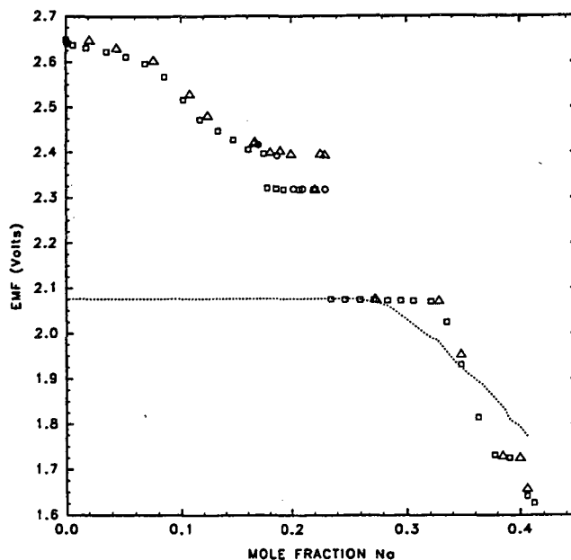
Figure 5. Plot of cell potential (EMF) vs Na mole fraction in P-S melt within sodium/phosphorous-sulfur cell. \square 1st discharge, \Delta charge, \circ discharge, — Na/S at 350°C
