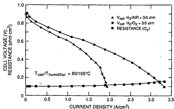
Figure 13a. Performance of a PEFC with a thin catalyst layer based on Pt/C catalyst bonded to the membrane. Loading - 0.17 mg Pt/cm 2 /electrode. The ionomeric membrane used here was membrane "C" (Chlorine Engineers, Japan).
