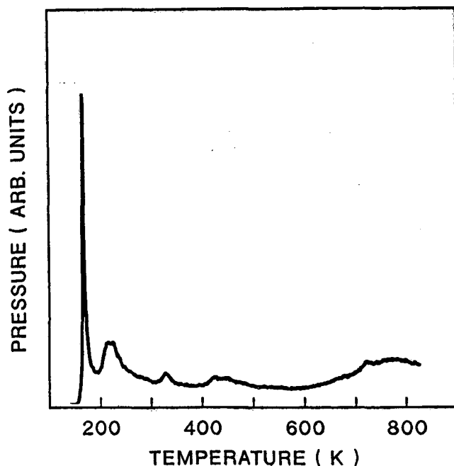
Figure 9. TPD spectrum of a Li-covered Ag surface exposed to 10 L D-THF at 98 K.
