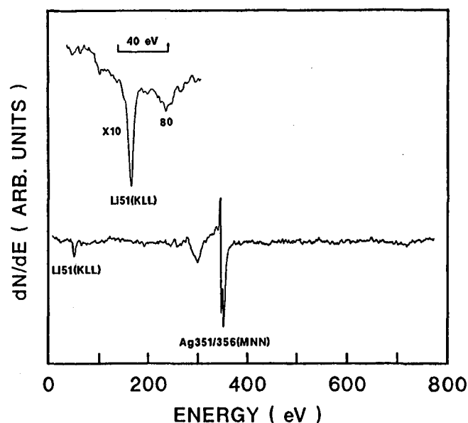
Figure 8. AES spectrum of a Li-covered Ag surface (50% Li). The inset displays another spectrum in the region of the Li(KLL) transition recorded at much higher sensitivity.
