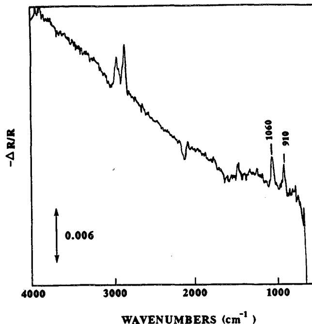
Figure 6. FTIRRAS spectrum of a Li-THF layer formed by simultaneous codeposition of the two constituents on a freshly coated Au surface at 90 K.
