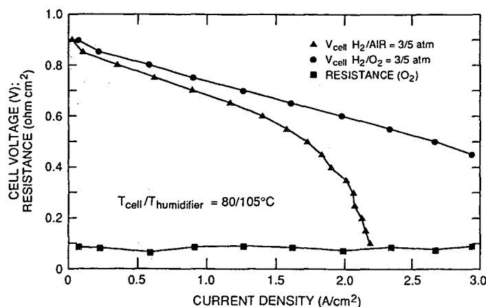
Figure 13b. Same as Fig. 13a for Pt loading of 0.13 mg Pt/cm 2 /electrode and an experimental Dow membrane.
