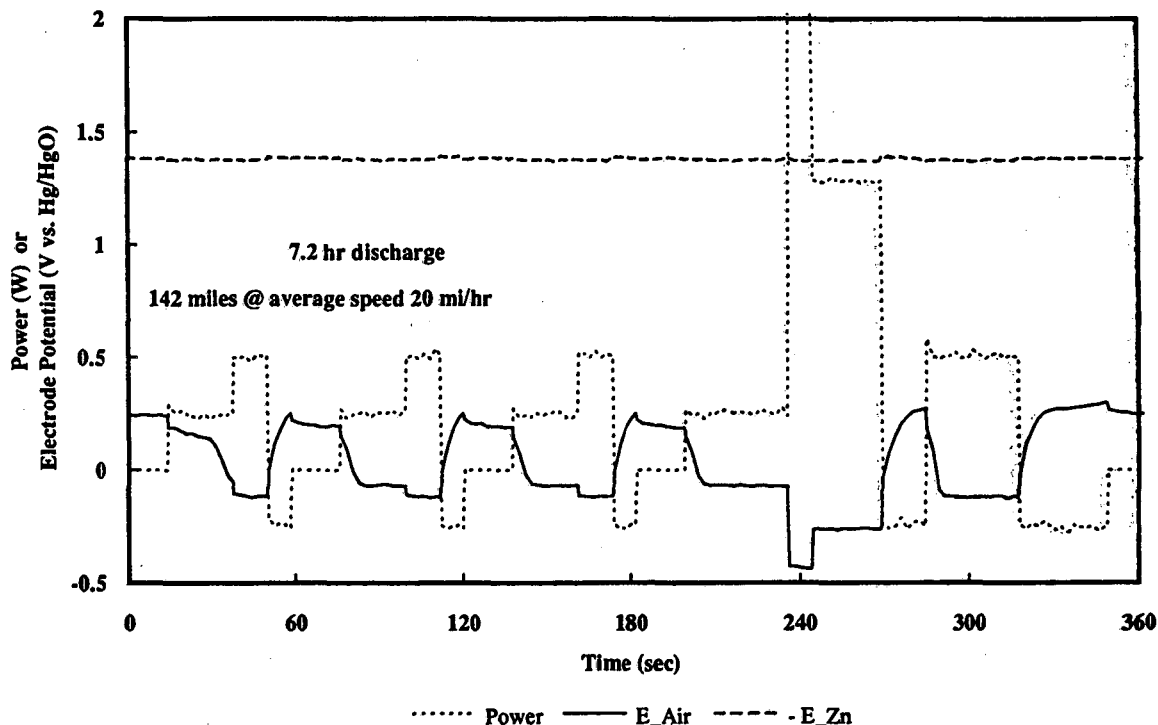
Figure 12. Discharge #6 of a 1.8 Ah Zn/air cell at SFUDS Repetition #40.
