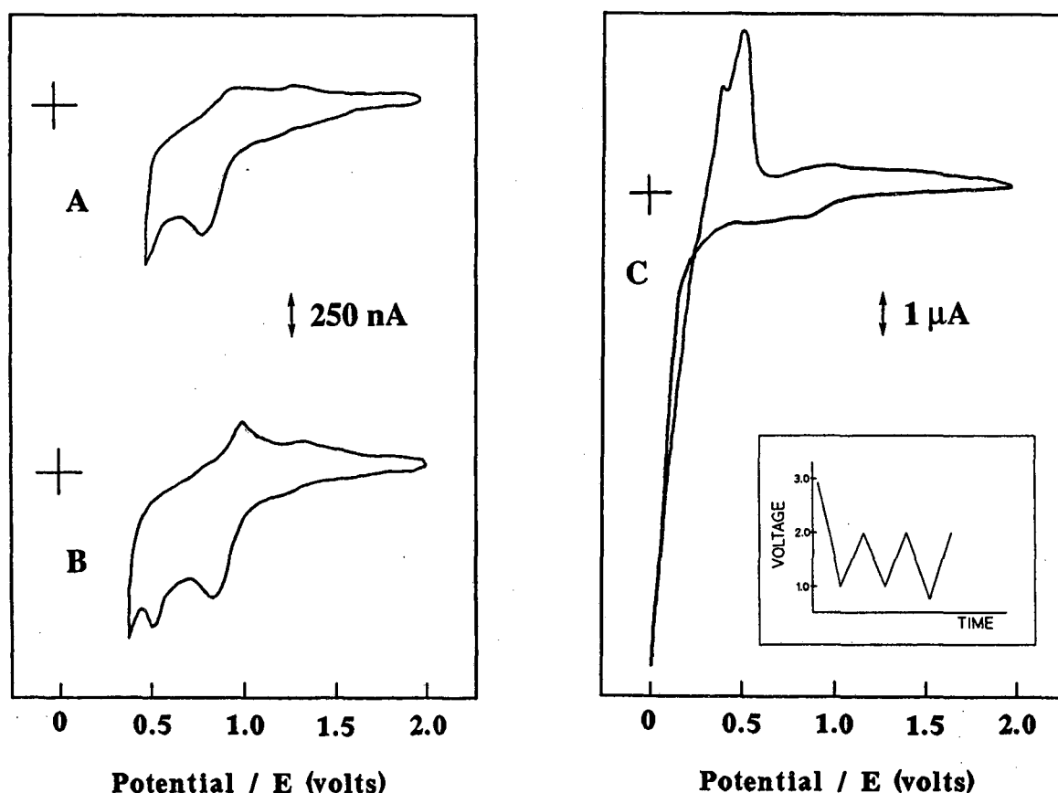
Figure 11. Series of voltammetric cycles obtained in sequence for a vapor-deposited Au electrode in \text{LiClO}_4/\text{PEO} at 55°C using a two-electrode cell configuration. Electrode Area: 0.31 \text{ cm}^2 . Curve A: Third Cycle; Curve B: Fourth Cycle; Curve C: Fifth Cycle. Prior to recording these curves, the electrode was cycled according to the program given schematically in the Insert.
