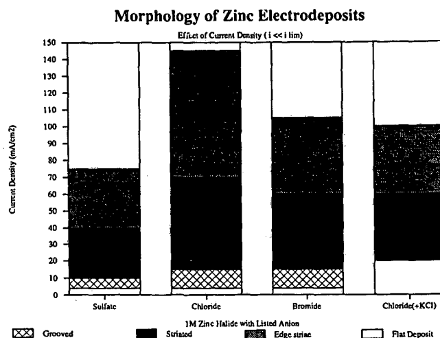
Figure 2. Macromorphology of Zn after deposition of 180 \text{ C/cm}^2 , as a function of current density and electrolyte composition. The range of current densities over which striae appear varies only slightly, depending on the presence of supporting electrolyte and on the degree of Zn complexation. (XBL 902-448)
