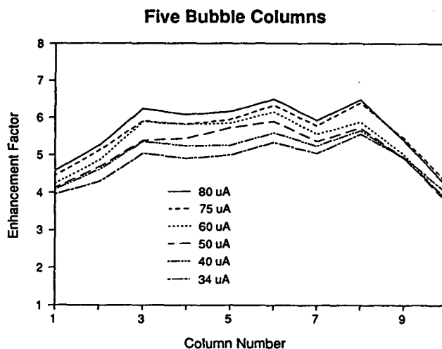
Figure 3. Enhancement of transport rates on vertically oriented micro-electrodes by curtain of five parallel hydrogen bubble streams. Distance between streams: 20 \mu\text{m} . Current densities at which bubbles were generated on satellite electrodes were 34 to 80 \text{ mA/cm}^2 . Peak enhancement is a factor of six higher than the natural convection limiting current. (XBL 915-1123)
