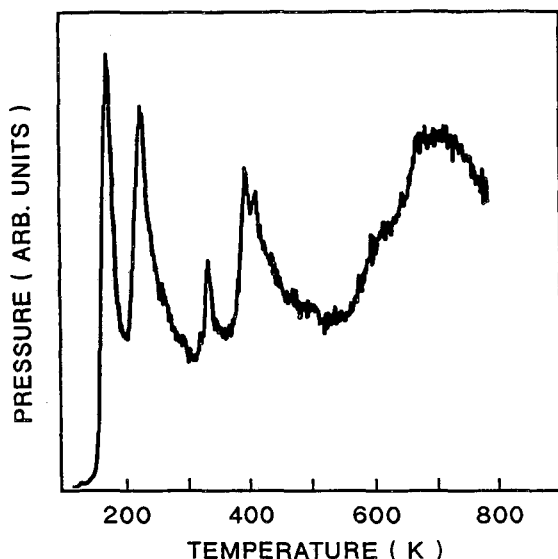
Figure 10. TPD spectrum of a Ag surface after exposure to 10 L of THF and Li at 98 K.
