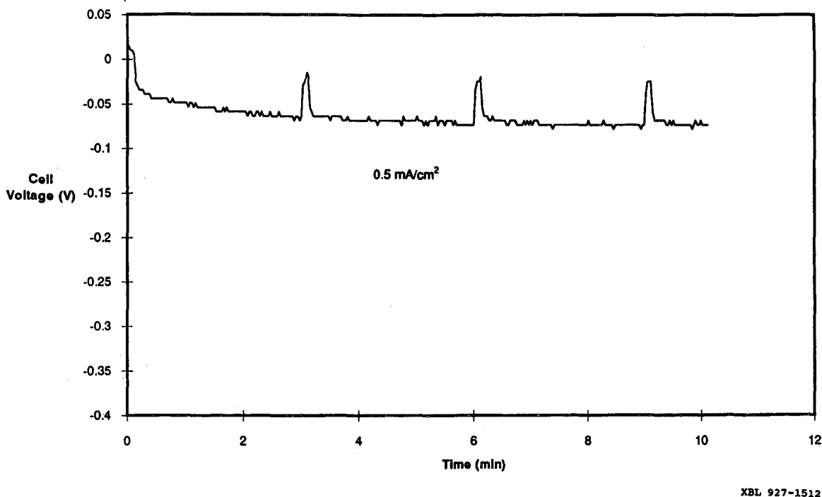
Figure 1. Discharge of Na/PEO-NaTf/Na cell at 0.5 mA/cm 2 .
