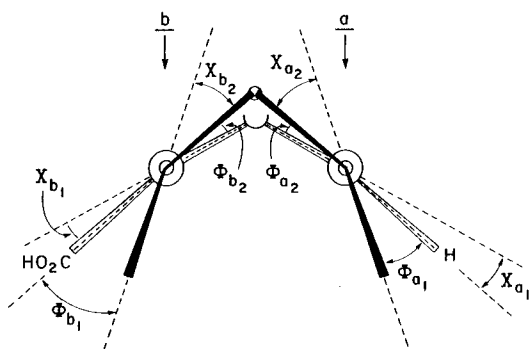
Fig. 3. Schematic representation of bridgehead diene 1 indicating pyramidalization ( \chi ) and torsion ( \phi ) at the bridgehead double bonds.
