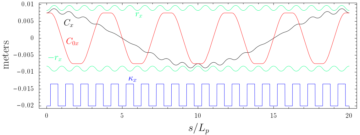
Figure 2.2: Comparison of depressed and undepressed principal orbits for \sigma_{0x} = 90^\circ and \sigma_x = 18^\circ . The red and black curves represent rescaled underessed and depressed x-plane cosine-like principal orbit functions, respectively. The matched beam envelope is plotted in green. The x-plane focusing function is plotted (arbitrary scale) in blue.
