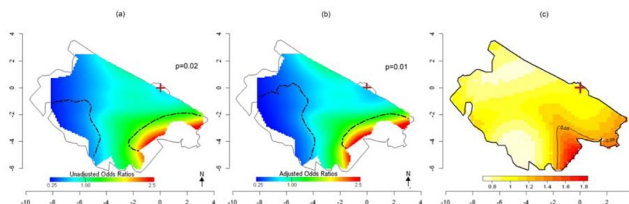
Fig 4. Spatial variation in of risk of HM death: Women only (86 cases and 168 controls) (a) Crude ORs for HM mortality using GAMs with optimal span=0.7. (b) ORs for HM mortality using GAMs adjusted for age and distance from power lines. Optimal span=0.65. Areas of significantly increased and decreased risk at the 0.025 level are denoted by black contour lines (c). Adaptive kernel Relative Risk of HM mortality estimation with 5% significant tolerance contours denoted by black contour lines. The brown cross marks the location of the refinery.
