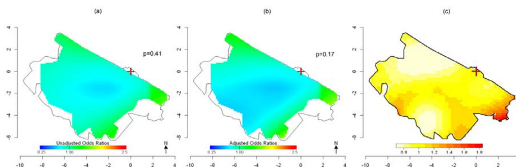
Fig 3. Spatial variation in mortality risk of HMs. All subjects (171 cases and 338 controls) (a) Crude ORs for HM mortality using GAMs with optimal span=0.95. (b) ORs for HM mortality using GAMs adjusted for sex, age and distance from power lines. Optimal span=0.95. (c) Adaptive kernel Relative Risk of HM mortality estimation. The brown cross marks the location of the refinery.
