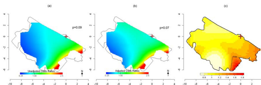
Fig 6. Spatial variation of risk of HM death: Women whose relatives were interviewed (49 cases and 123 controls)
