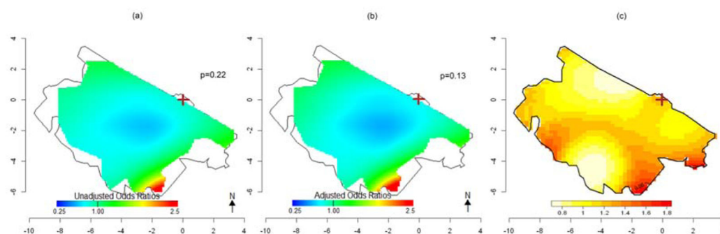
Fig 5. Spatial variation in risk of HM death: Subjects whose relatives were interviewed (101 cases and 249 controls)
