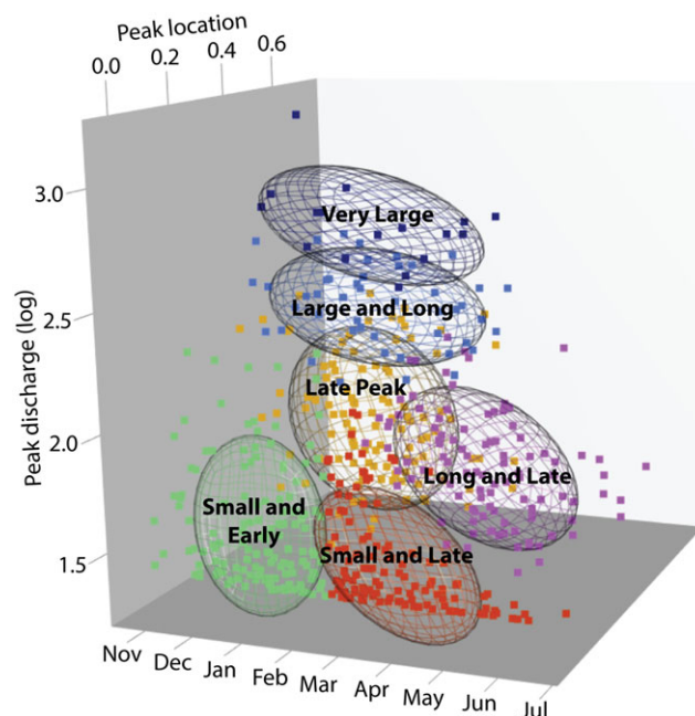
FIGURE 3 Clustered flood events along three metrics used in analysis: magnitude of peak discharge (log transformed), centroid date, and location of hydrograph peak (fraction of flood-event duration before the day of peak flow). Ellipses cover the 50% confidence region for each type. The color scheme is consistent across figures
