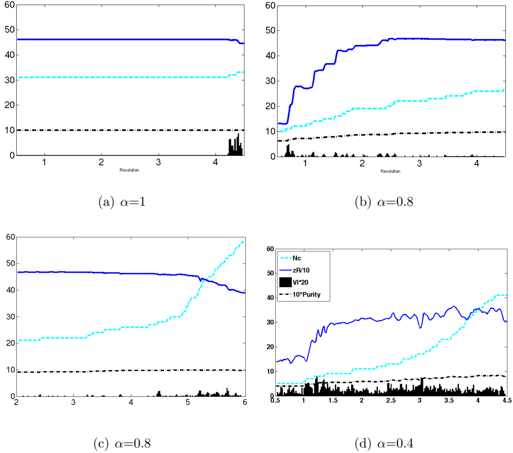
Figure 3.4: Partitioning results using the multi-slice modularity optimization, with \omega = 1 and \mathbf{W}_{GT} = \alpha\mathbf{T} + (1 - \alpha)\mathbf{G} . The number of clusters ( N_c ), zRand-score ( zR ) and purity ( Prt ) for the partition of each slice are plotted as functions of the resolution parameter \gamma_s . Different values of \alpha is used: (a) \alpha = 1 , (b) \alpha = 0.8 , (c) \alpha = 0.8 , and (d) \alpha = 0.4 .
