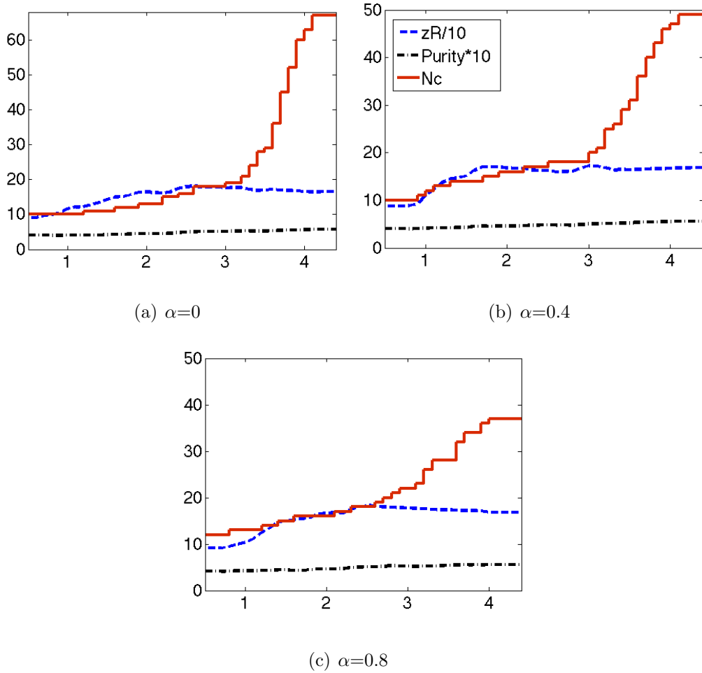
Figure 3.3: Partitioning results using the multi-slice modularity optimization, with \omega = 1 and \mathbf{W} = \alpha\mathbf{S} + (1 - \alpha)\mathbf{G} . The number of clusters ( N_c ), zRand-score ( zR ) and purity ( Prt ) for the partition of each slice are plotted as functions of the resolution parameter \gamma_s . Different values of \alpha is used: (a) \alpha = 0 , (b) \alpha = 0.4 , (c) \alpha = 0.8 .
