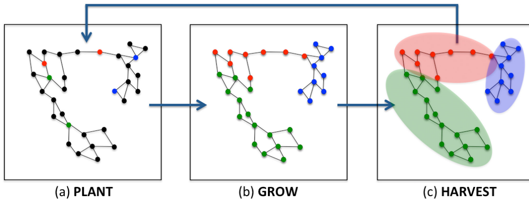
Figure 6.1: Illustration of the Incremental Reseeding (INCREAS) Algorithm for R = 3 clusters. The various colors red, blue, and green identify the clusters. (a): At this stage of the algorithm, s = 2 seeds are randomly planted in the clusters computed from the previous iteration. (b): The seeds grow with the random walk operator. (c): A new partition of the graph is obtained and used to plant s + ds seeds into these clusters at the next iteration.
