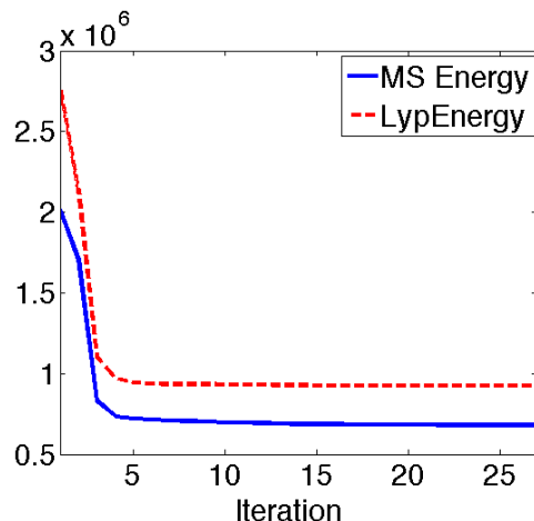
Figure 5.4: Energy MS(f) (blue, solid line) and Y_\tau(f) (red, dash line) at each iteration from the same test as shown in Figure 5.3 (a).
