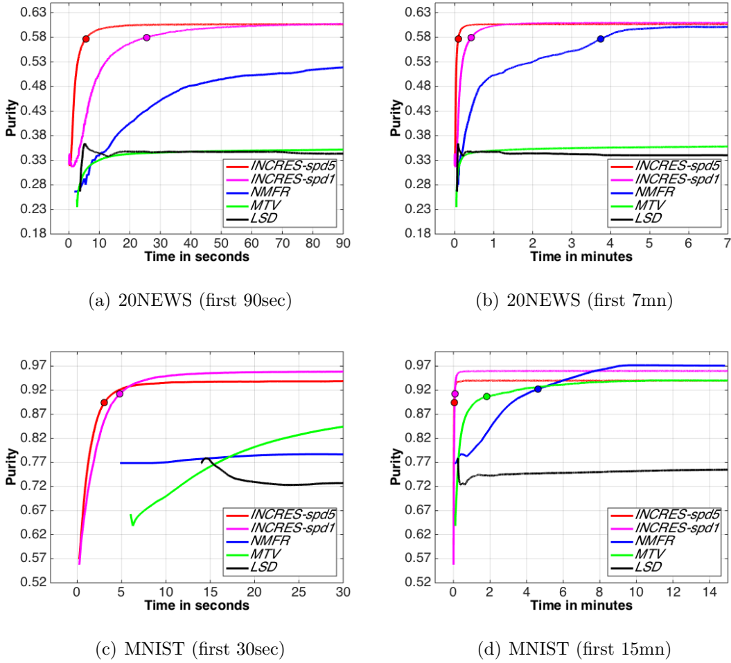
Figure 6.3: Purity curves for the four algorithms considered on two benchmark data sets (20NEWS and MNIST). We plot purity against time for each algorithm over two different time windows. The circular marks on each curve indicate the point at which the curve reaches 95% of its limiting value. The corresponding times at which this happens are reported in Table 6.2.
