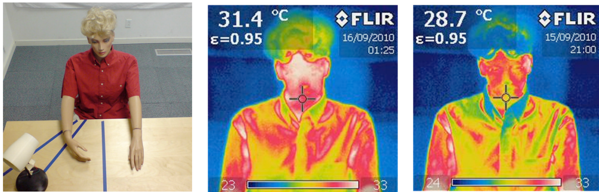
Manikin test with a PEC fan
