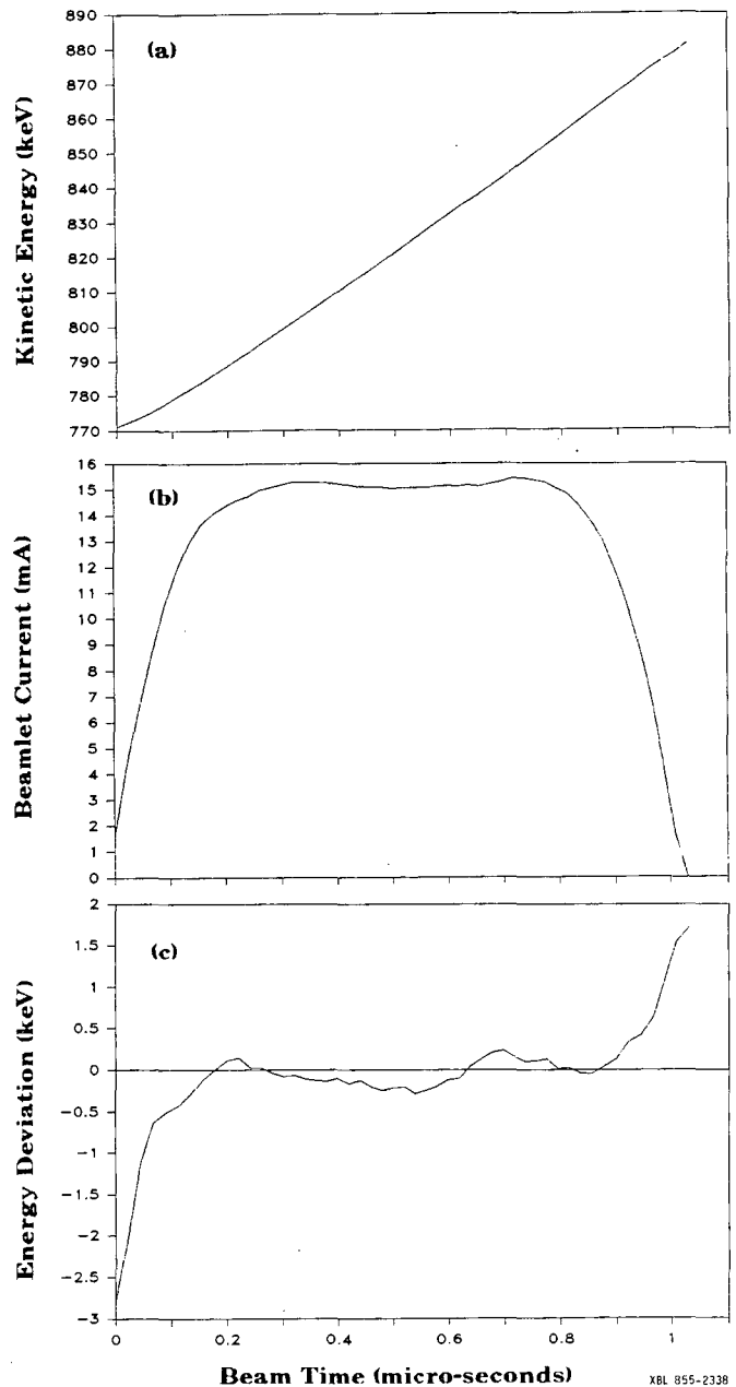
Fig. 4 (a) Kinetic energy of the bunch, (b) Current, and (c) Energy Deviation -- compared to the "ideal values" -- as functions of beam time at the exit end of MBE-4. Input current is 5 mA per beamlet at 200 keV.
