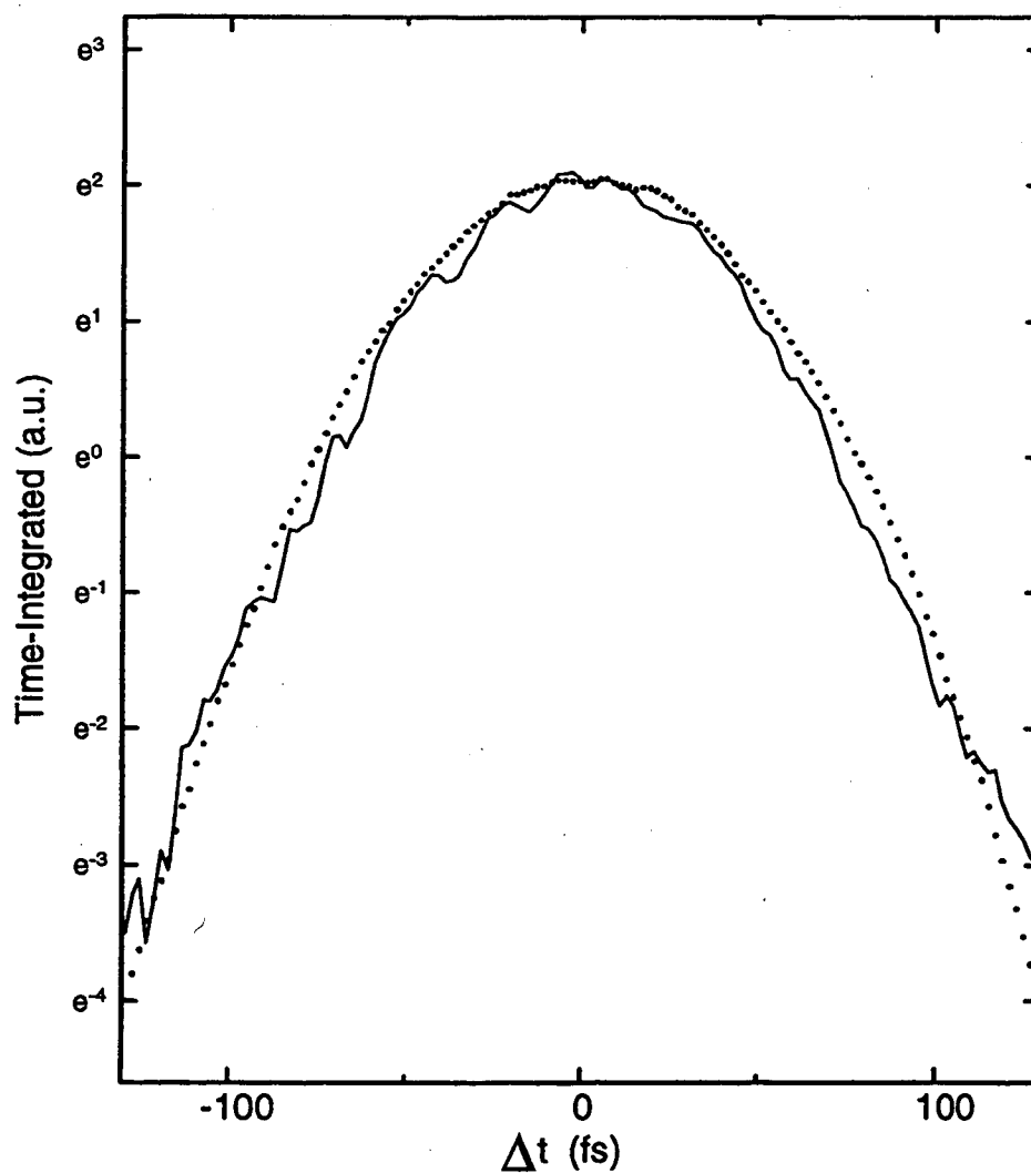
Figure 5.1: TI SWM lineshape measured at high excitation density N_x \approx 10^{13} \text{cm}^{-2} (solid curve) compared with the noncolinear autocorrelation trace of the excitation laser pulse raised to the power 5/2 (dotted curve).
