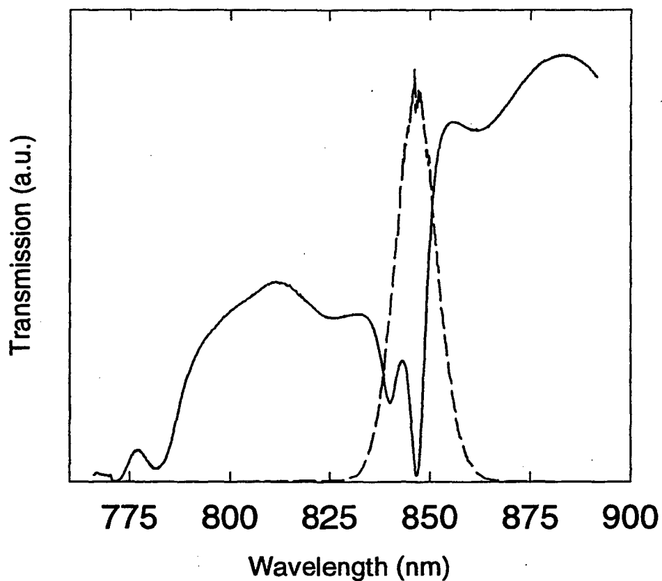
Figure 4.1: Transmission spectrum of the multiple quantum well sample at room temperature (solid line) and the power spectrum of the excitation laser pulse (dashed line). The pronounced dips in the transmission at approximately 840nm and 846nm are the n=1 light-hole and heavy-hole excitons, respectively.
