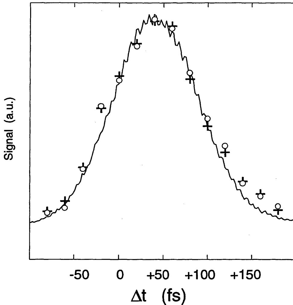
Figure 4.7: TI FWM signal measured directly with the GaAs slow detector (solid line). Numerical integration (crosses) and maximum amplitude (hollow circles) of the TR FWM data shown in Fig.4.3. All data points are normalized to the peak of the TI FWM signal and all data are taken at excitation density N_x \approx 3 \times 10^{11} \text{ cm}^{-2} and with an excitation laser pulse duration of (78 \pm 3) \text{ fs} .
