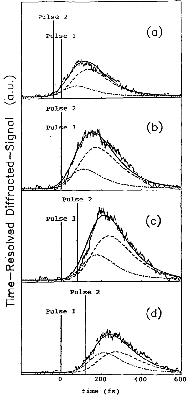
Figure 4.10: Numerical fits to TR FWM data taken at excitation density N_x \approx 10^{11} \text{ cm}^{-2} and with an excitation laser pulse duration of (98 \pm 2) fs for time-delays \Delta t = (a)-40 fs, (b)0 fs, (c)+80 fs, (d)+120 fs. The dash-dotted lines give the phase-space filling contribution, the dashed lines give the Coulomb contribution, and the solid lines give their sum.
