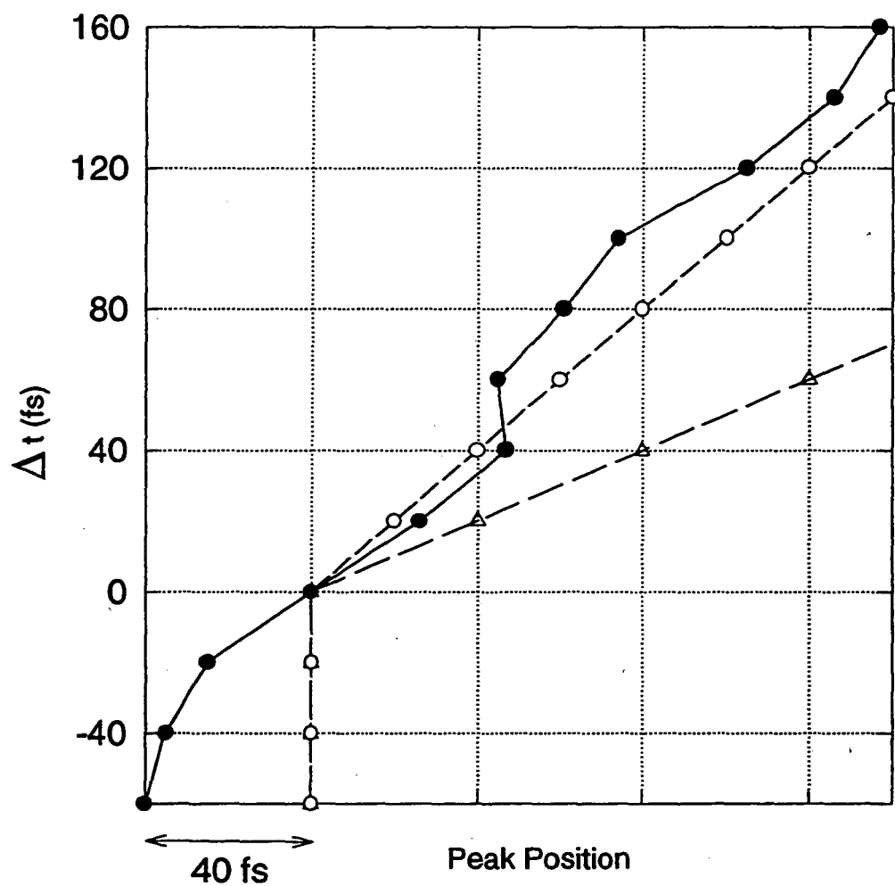
Figure 4.6: Relative positions of the maxima of the TR FWM signals shown in Fig.4.5 vs. time delay \Delta t (filled circles). Evolution expected for free induction decay signals (hollow circles) and for photon echoes (triangles).
