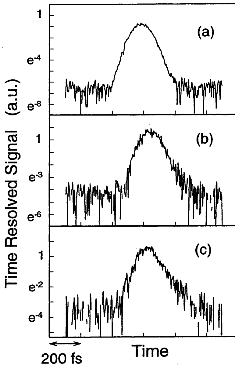
Figure 5.3: TR SWM lineshapes measured at \Delta t = 0 for excitation densities (a) N_x \approx 10^{13} \text{ cm}^{-2} , (b) N_x \approx 4 \times 10^{12} \text{ cm}^{-2} , and (c) N_x \approx 2 \times 10^{12} \text{ cm}^{-2} . The dephasing times extracted from the TR decays are: (a) T_2 \approx 54 \text{ fs} ; (b) T_2 \approx 84 \text{ fs} ; (c) T_2 \approx 132 \text{ fs} .
