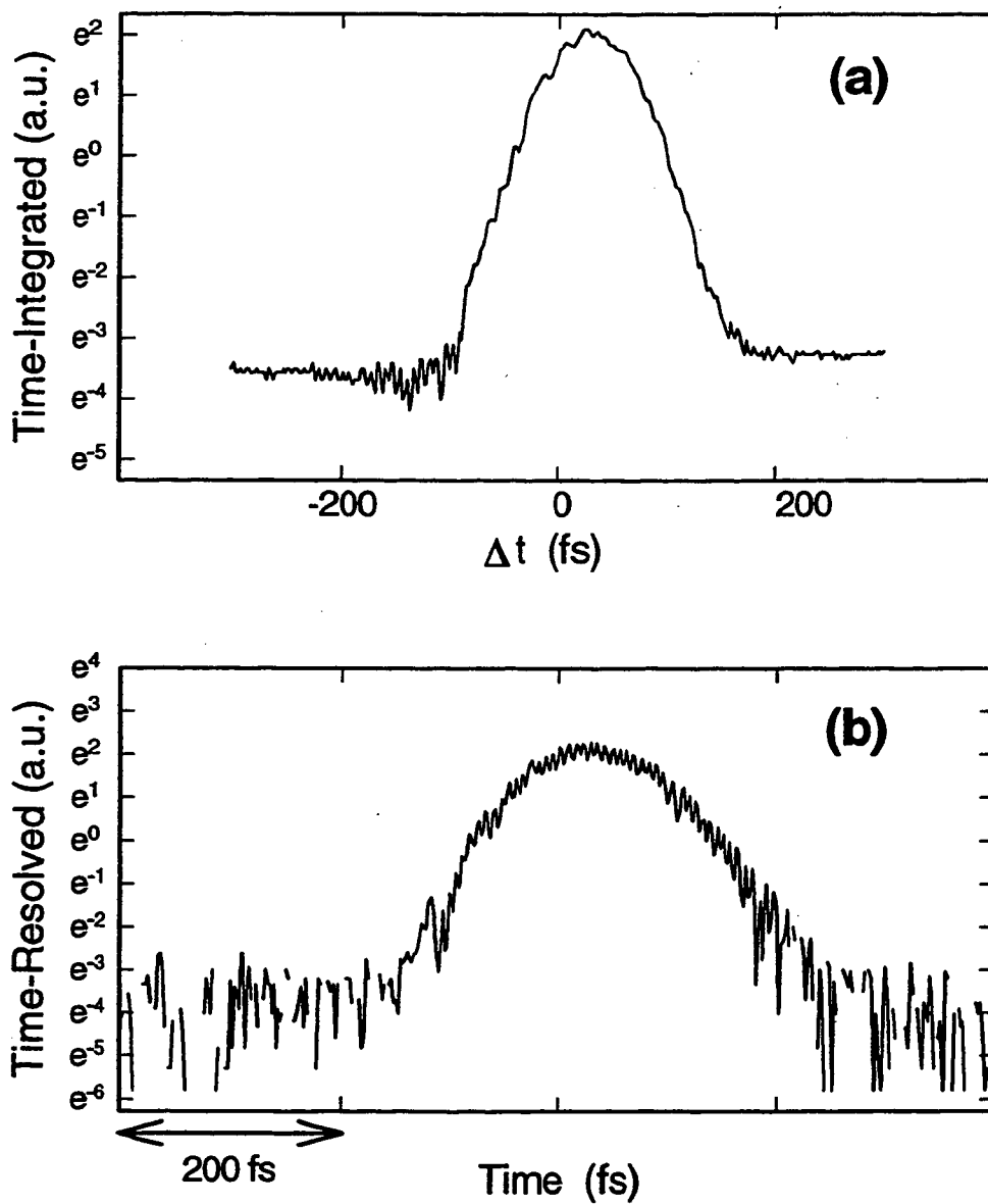
Figure 5.2: Symmetric TI SWM lineshape (a) vs. asymmetric TR SWM lineshape at \Delta t = +80 fs (b). All data were taken at high excitation density N_x \approx 10^{13} \text{ cm}^{-2} .
