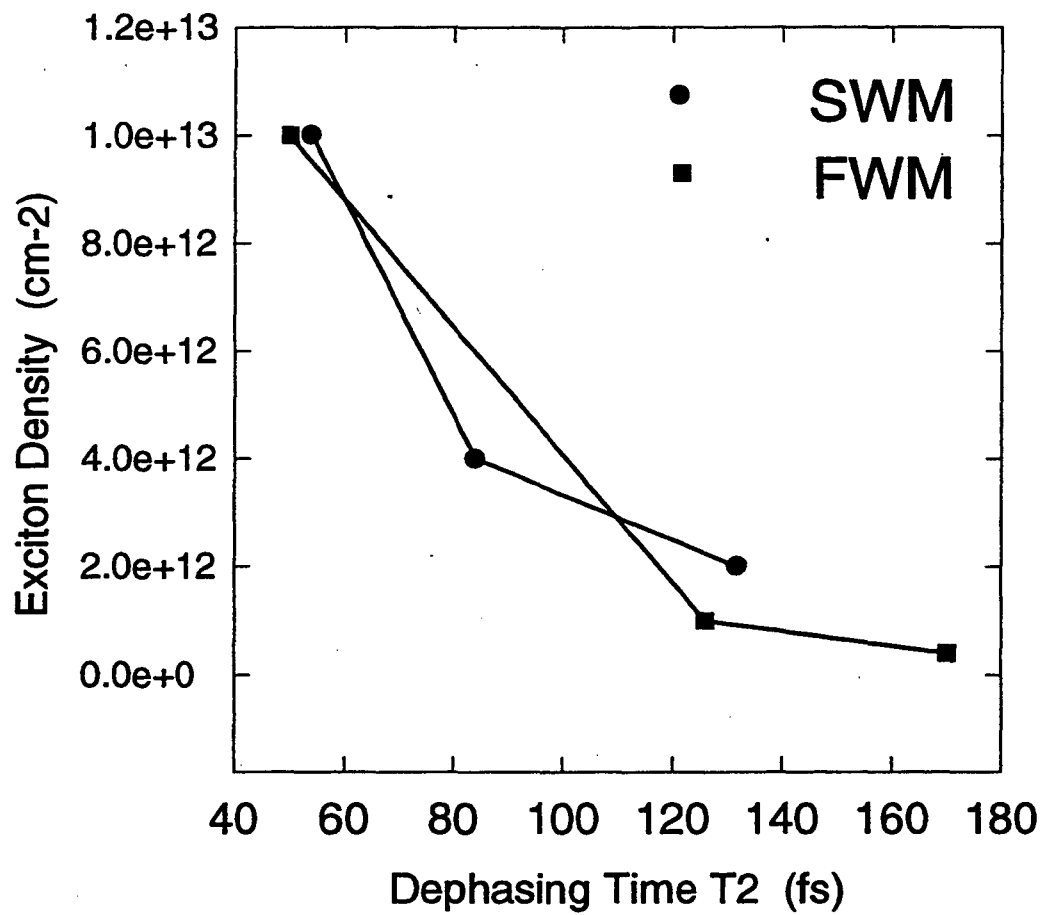
Figure 5.4: Comparison of dephasing times T_2 extracted from SWM (circles) and FWM (squares) measurements for several excitation densities.
