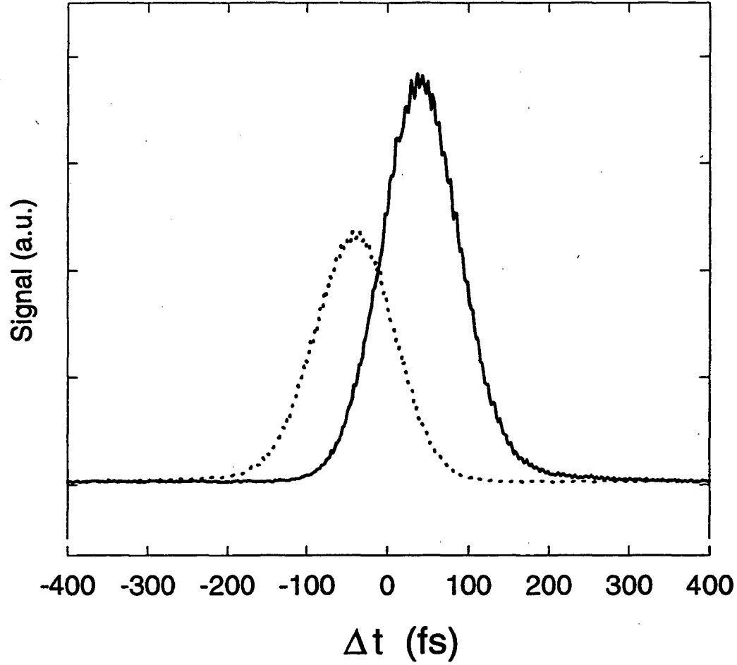
Figure 4.2: Finding time delay \Delta t = 0 using the intersection of TI FWM signals from directions 2k_1-k_2 (dotted line) and 2k_2-k_1 (solid line), for typical experimental conditions: excitation density N_x \approx 3 \times 10^{11} \text{ cm}^{-2} and laser pulse duration (78 \pm 3) \text{ fs} .
