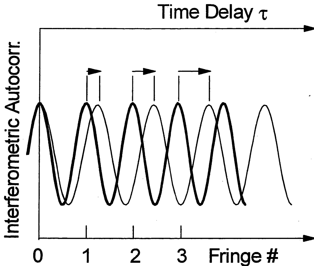
Figure 3.7: The differential fringe spacing DFS(\tau) (magnitude shown by arrows) is determined by comparing the position of interferometric autocorrelation fringes of the signal pulse (thin line) with the position of the corresponding fringes of the reference pulse from the laser (thick line). The case of “linear chirp” is sketched here.
