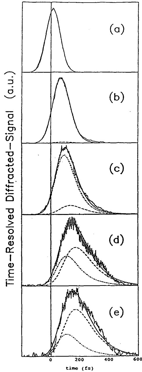
Figure 4.11: Numerical fits to the TR FWM data taken at \Delta t = 0 and for a series of excitation densities N_x \approx (a) 10^{13} , (b) 10^{12} , (c) 4 \times 10^{11} , (d) 2 \times 10^{11} , and (e) 10^{11} \text{ cm}^{-2} . The dash-dotted lines give the phase-space filling contribution, the dashed lines give the Coulomb contribution, and the solid lines give their sum.
