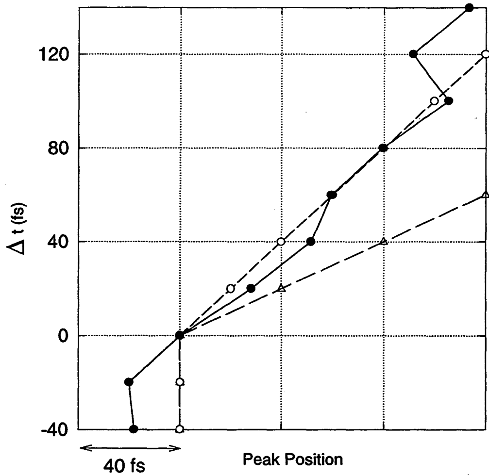
Figure 4.4: Relative positions of the maxima of the TR FWM signals shown in Fig.4.3 vs. time delay \Delta t (filled circles). Evolution expected for free induction decay signals (hollow circles) and for photon echoes (triangles).
