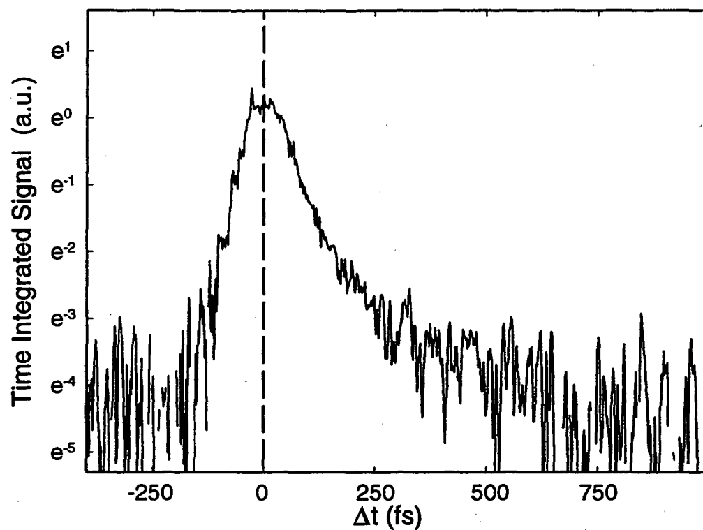
Figure 5.5: TI SWM trace at low excitation density N_x \approx 2.7 \times 10^{11} \text{ cm}^{-2} . The dashed line is a visual aid to demonstrate the asymmetry of the curve.
