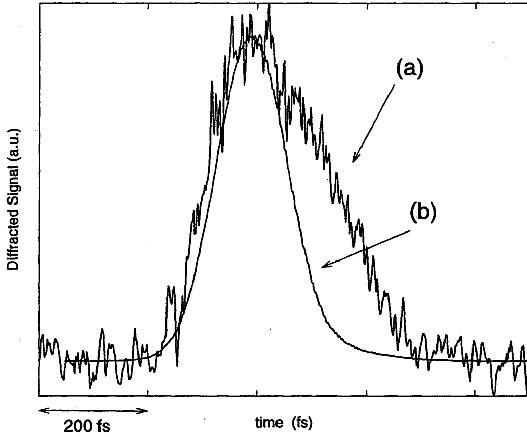
Figure 4.8: (a) TR FWM signal recorded for \Delta t = 0 and (b) the corresponding TI FWM signal. All data are taken for excitation density N_x \approx 10^{11} \text{ cm}^{-2} and with an excitation laser pulse duration of (96 \pm 2) \text{ fs} .
