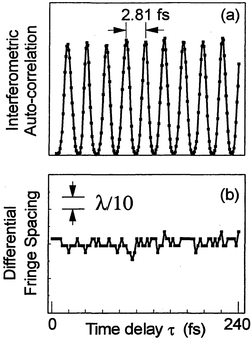
Figure 3.6(a): The resolution of the interferometric measurement is determined by the number of steps per fringe (21) and the duration of the optical cycle (2.81 fs), giving a minimum time-delay smaller than 140 attoseconds.
