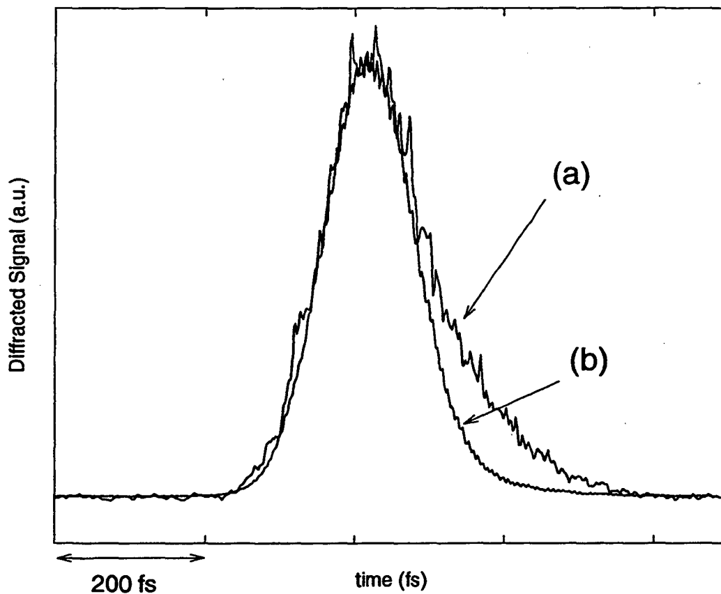
Figure 4.9: (a) TR FWM signal recorded for \Delta t = 0 and (b) the corresponding TI FWM signal. All data are taken for excitation density N_x \approx 4 \times 10^{11} \text{ cm}^{-2} and with an excitation laser pulse duration of (98 \pm 2) \text{ fs} .
