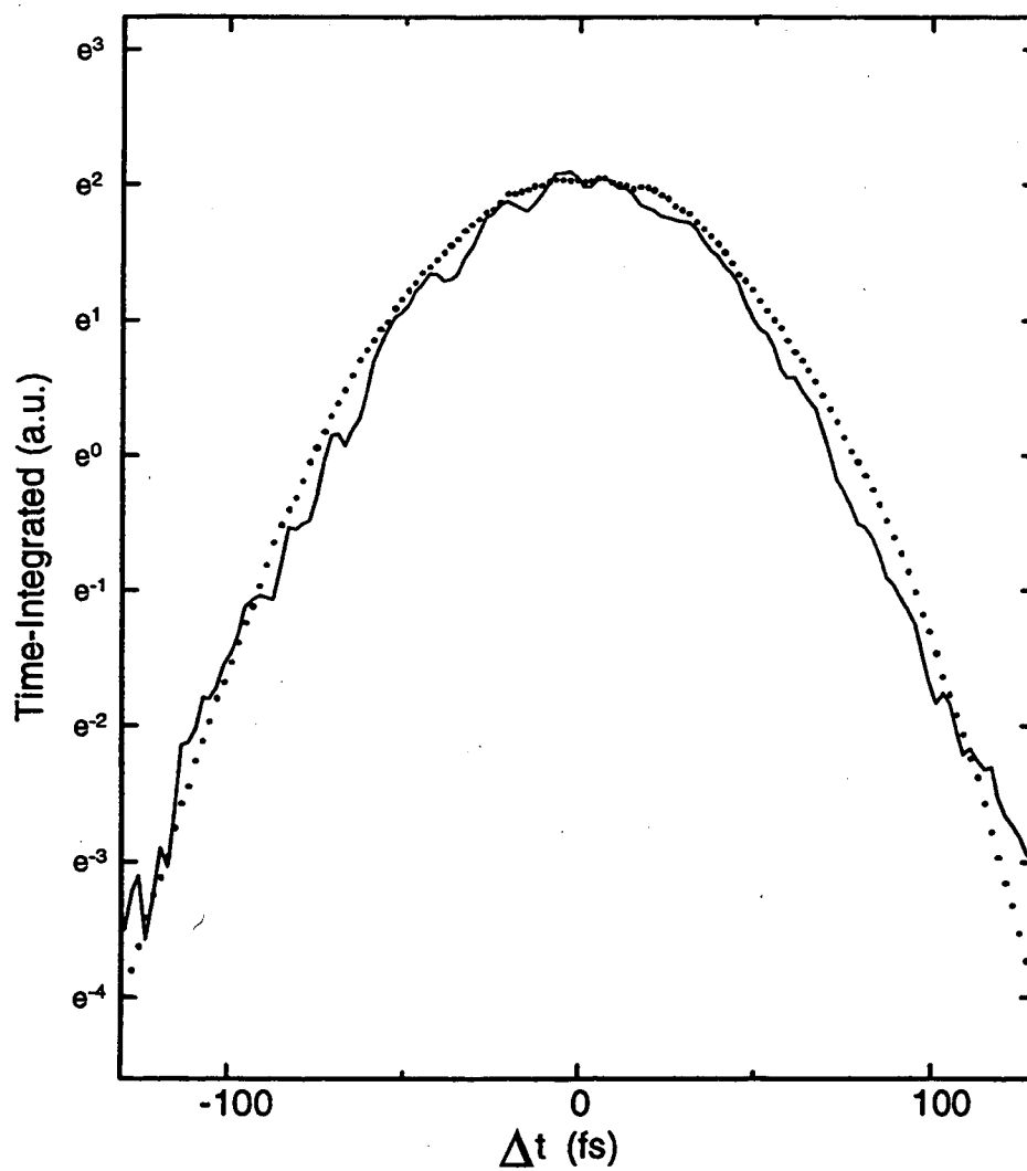
Figure 5.1: TI SWM lineshape measured at high excitation density N_x \approx 10^{13} \text{ cm}^{-2} (solid curve) compared with the noncolinear autocorrelation trace of the excitation laser pulse raised to the power 5/2 (dotted curve).
