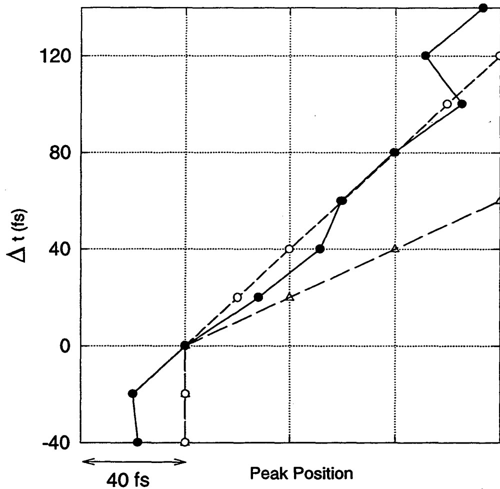
Figure 4.4: Relative positions of the maxima of the TR FWM signals shown in Fig.4.3 vs. time delay \Delta t (filled circles). Evolution expected for free induction decay signals (hollow circles) and for photon echoes (triangles).
