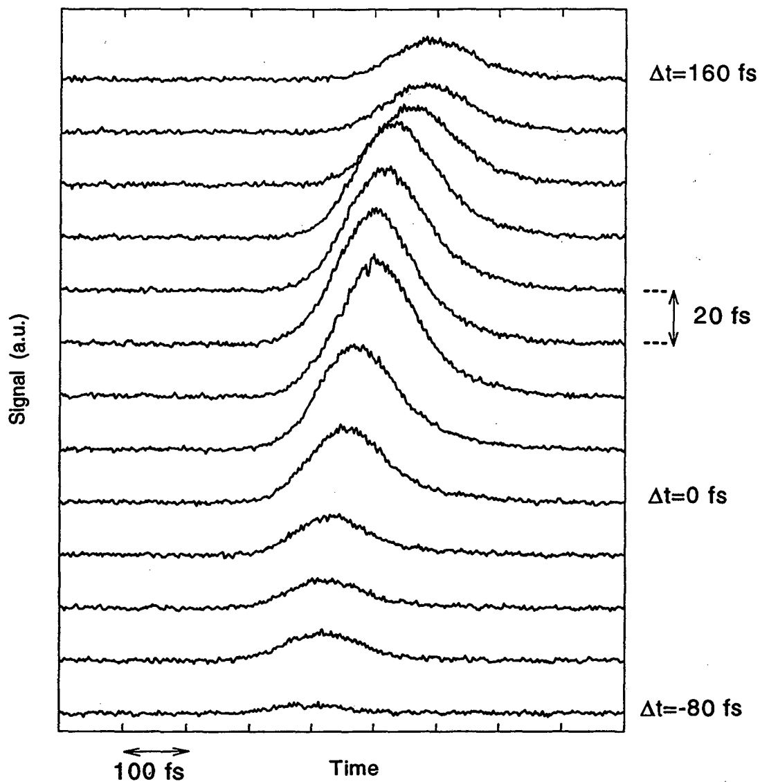
Figure 4.5: TR FWM signals, offset for clarity, for a range of time delays \Delta t between -80fs and +160fs. The data were taken for an excitation density N_x \approx 10^{12} \text{cm}^{-2} and for an excitation laser pulse duration of (78 \pm 3) \text{fs} .
