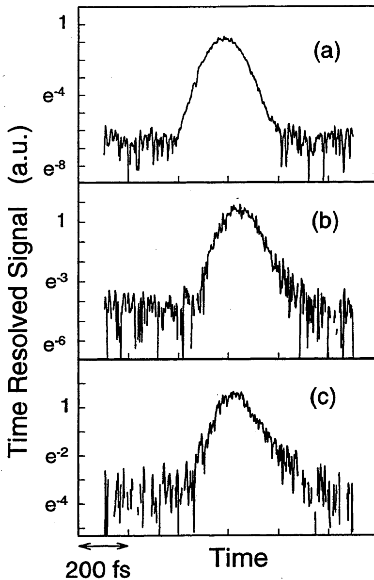
Figure 5.3: TR SWM lineshapes measured at \Delta t = 0 for excitation densities (a) N_x \approx 10^{13} \text{cm}^{-2} , (b) N_x \approx 4 \times 10^{12} \text{cm}^{-2} , and (c) N_x \approx 2 \times 10^{12} \text{cm}^{-2} . The dephasing times extracted from the TR decays are: (a) T_2 \approx 54 \text{fs} ; (b) T_2 \approx 84 \text{fs} ; (c) T_2 \approx 132 \text{fs} .
