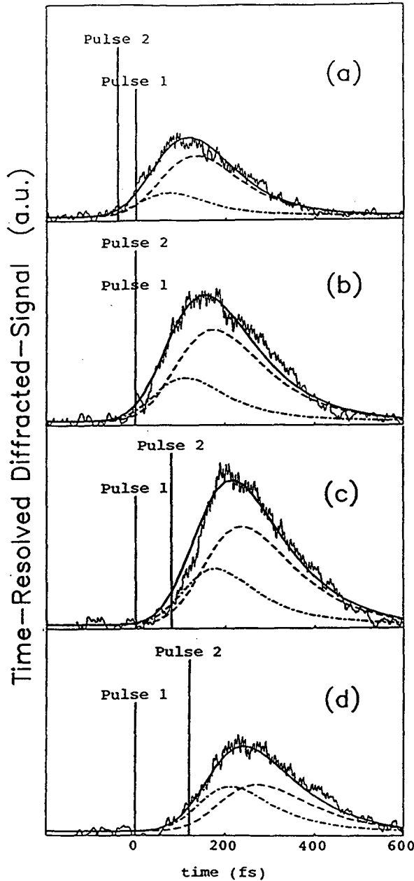
Figure 4.10: Numerical fits to TR FWM data taken at excitation density N_x \approx 10^{11} \text{cm}^{-2} and with an excitation laser pulse duration of (98 \pm 2) fs for time-delays \Delta t = (a)-40 fs, (b)0 fs, (c)+80 fs, (d)+120 fs. The dash-dotted lines give the phase-space filling contribution, the dashed lines give the Coulomb contribution, and the solid lines give their sum.
