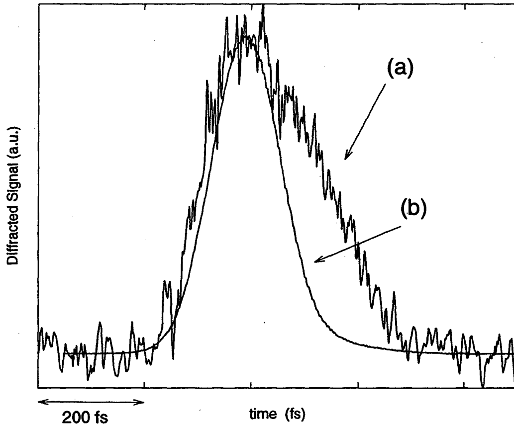
Figure 4.8: (a) TR FWM signal recorded for \Delta t = 0 and (b) the corresponding TI FWM signal. All data are taken for excitation density N_x \approx 10^{11} \text{cm}^{-2} and with an excitation laser pulse duration of (96 \pm 2) \text{fs} .
