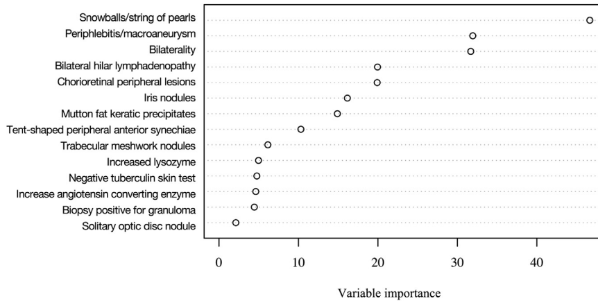
Figure 1. Random forest-based variable importance analysis of tests included in the latent class model with 2 classes for classifying the latent classes.
