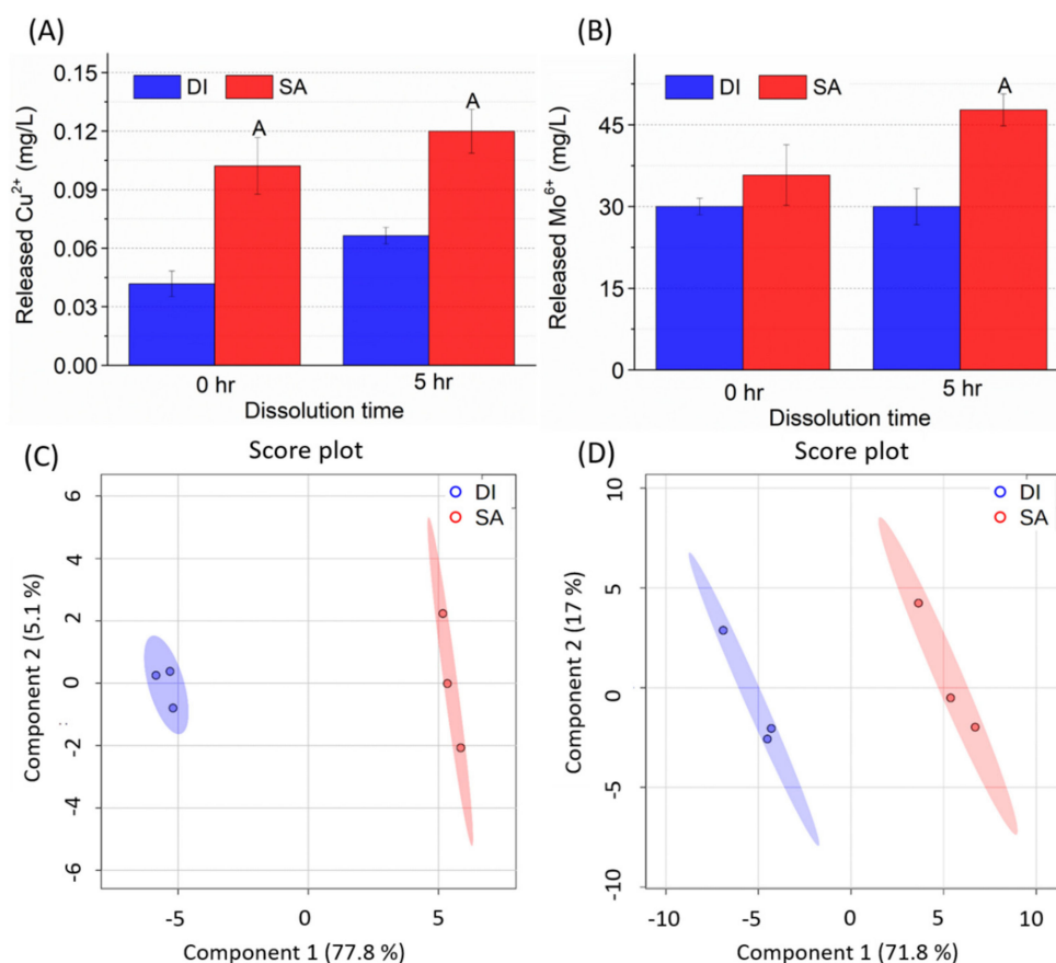
Figure 1. Metal ions released from (A) 100 mg/L Cu(OH) 2 NMs and (B) 100 mg/L MoO 3 NMs in DI water (DI) and surfactant containing suspensions (SA). PLS-DA score plots of overall metabolites in wheat (C) leaves and (D) roots after one-week foliar exposure to DI and SA solutions. Three replicates were used under each condition.
