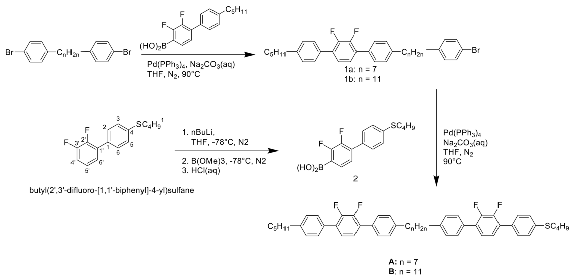
Figure 1: Scheme of the Synthesis of the investigated systems A and B .
