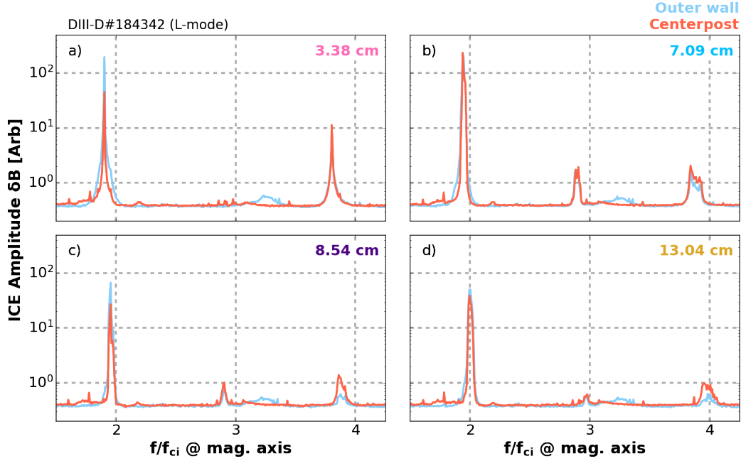
Figure 5.6: Centerpost (red) and outer wall loop (light blue) autopowers time-averaged over 2.5 MW, on-axis beam pulses at gapout values of (a) 3.38, (b) 7.09, (c) 8.54, and (d) 13.04 cm as denoted in Fig. 5.5. f_{ci} is the deuterium ion cyclotron frequency evaluated at the magnetic axis.
