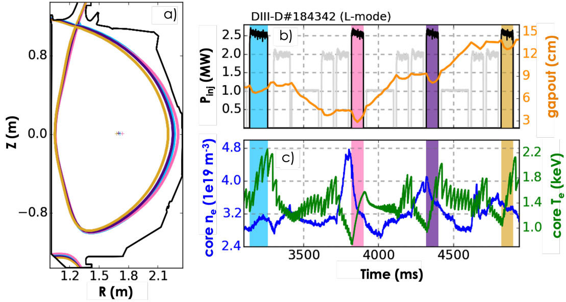
Figure 5.5: (a) Plasma equilibria at different gapout values. (b) Injected power from the 2.5 MW co\text{-}I_P neutral beam (black) and gapout parameter (orange) with gapout values of interest marked by colored rectangles.
