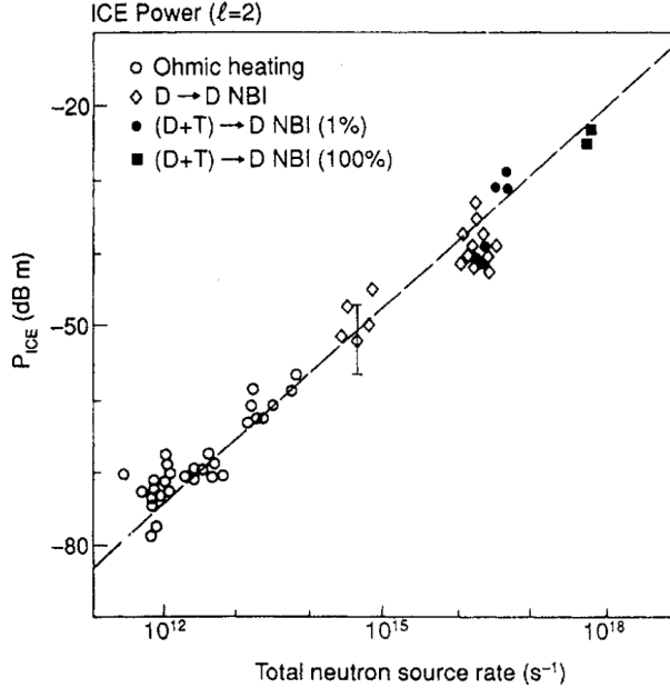
Figure 2.1: ICE power ( P_{\text{ICE}} ) vs. neutron rate in both ohmic and NBI-heated JET plasmas, where the dependence is nearly linear ( P_{\text{ICE}} \propto R_{\text{neutrons}}^{0.9 \pm 0.1} ). Figure taken from [37].
