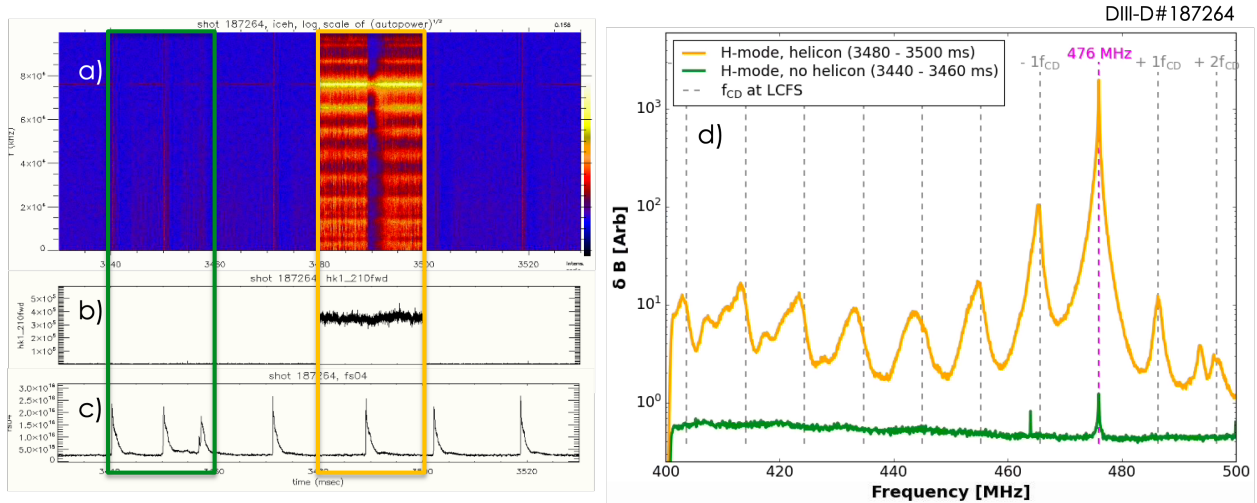
Figure C.5: (a) Autopower spectra from the outer wall loop during the H-mode period in DIII-D#187264, with forward helicon power depicted in (b) and D- \alpha signal in (c). The autopower data averaged over time windows during negligible (green) and \sim 350 kW (gold) of helicon forward power are presented in (d).
