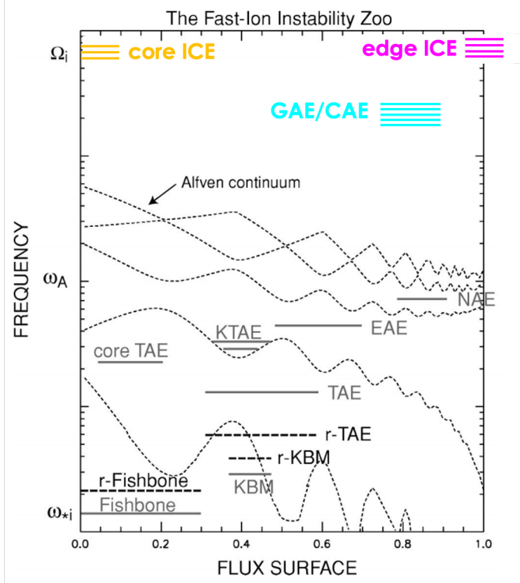
Figure 1.6: EP modes observed in tokamaks in terms of approximate frequency, location, and mode width. Of particular interest in this work are high-frequency modes such as CAEs and ICE. Figure taken from [77].
