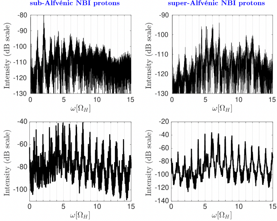
Figure 2.14: Comparison of measured ICE spectra (top panels) and simulated ICE (bottom) in LHD for super- and sub-Alfvénic ions. Figure taken from [136].
