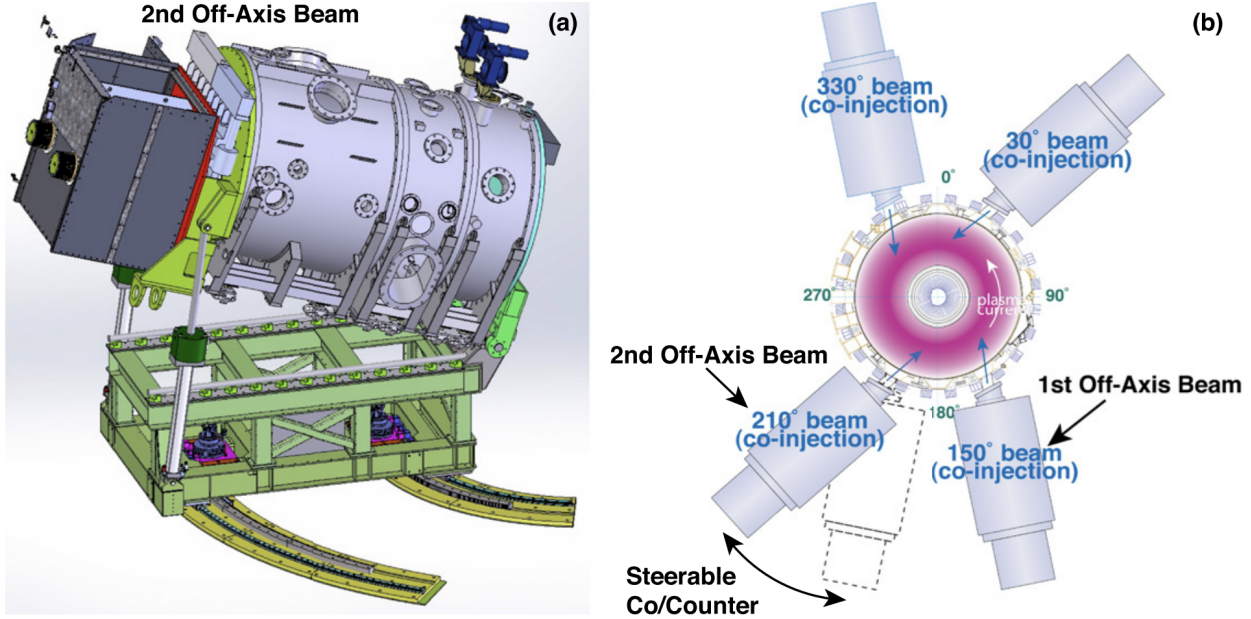
Figure 3.2: (a) Rendering of the 210^\circ beam that was tilted off-axis permanently in 2019, alongside (b) an aerial view of the DIII-D beams. Figure taken from [75].
