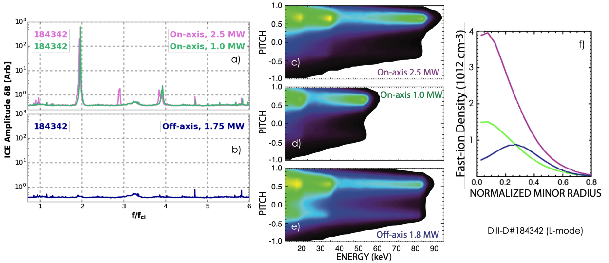
Figure 4.4: Time-averaged autopower spectrum over the course of a 100 ms pulse from co-I_P , co-tangential beams, which were (a) on-axis at 30° and 330° and (b) off-axis at 150°. f_{ci} is evaluated at the magnetic axis. The fast ion distribution velocity profile for each beam pulse is depicted in (c), (d), and (e), where the relative value of the color scale is 1.0, 0.60, and 0.24, respectively. The spatial profile, taken by summing the fast ion distributions in velocity space, is presented in (f).
