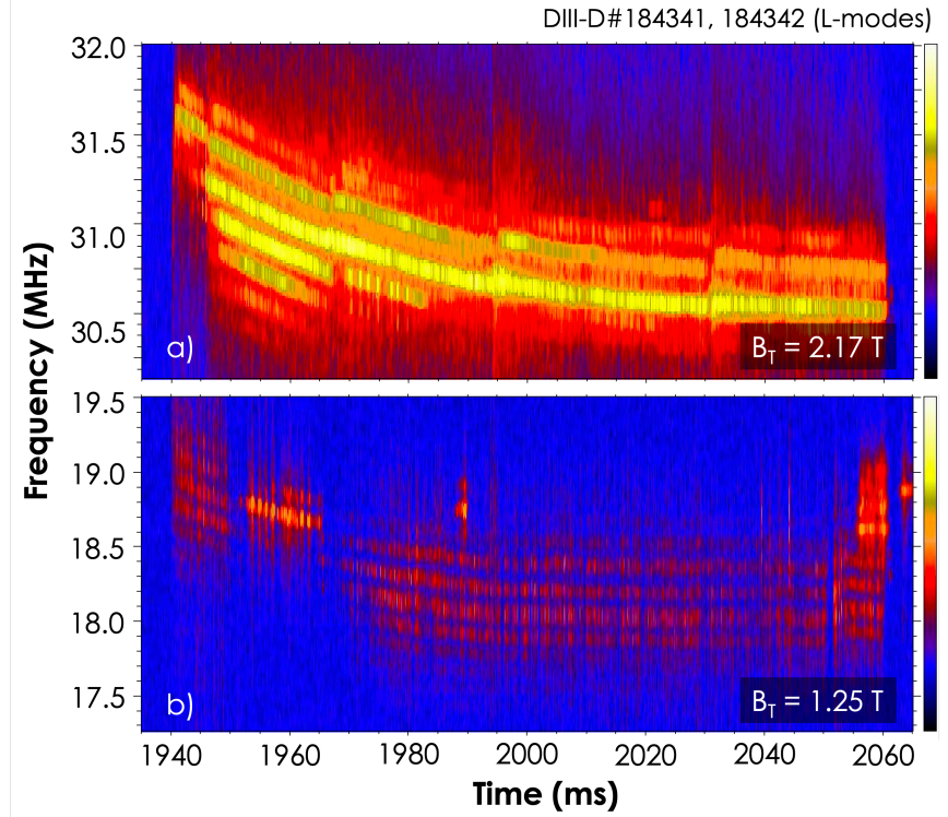
Figure 5.16: Second harmonic core ICE excited by the same on-axis, near-tangential, co\text{-}I_P 2.5 MW beam in a) B_T = 2.17 T and b) 1.25 T L-mode plasmas.
