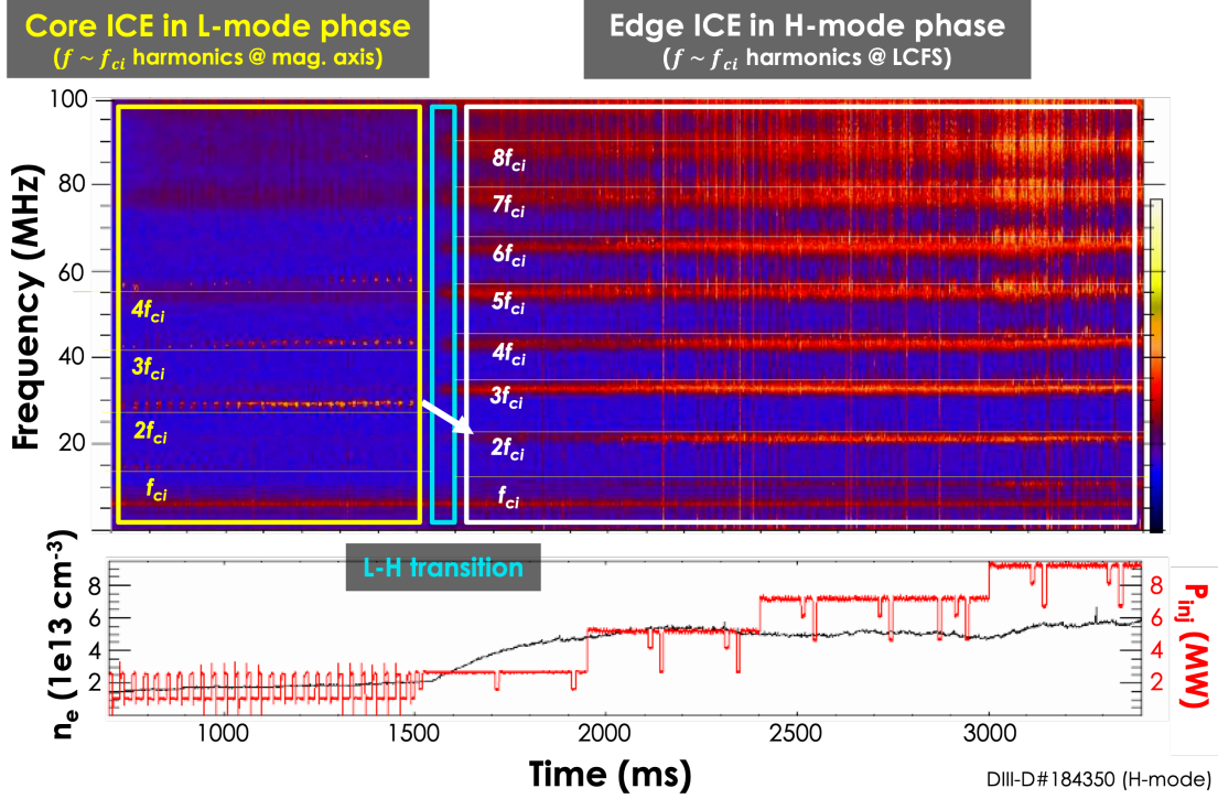
Figure 4.3: (a) An example of an H-mode shot exhibiting both core and edge-localized ICE, where horizontal lines have been overlaid to indicate f_{ci} evaluated at the magnetic axis in L-mode (yellow) and the LCFS in H-mode (white). The shot begins in L-mode (left), with the neutral beams exciting core ICE harmonics 1–4 f_{ci} . After the L-H transition, harmonics 1–9 f_{ci} are excited and localized near the plasma edge. Noise at roughly 5 MHz is observed throughout the discharge and is likely caused by the power supplies. (b) NBI power (MW) in red and electron density n_e ( 1e13 \text{ cm}^{-3} ) in black.
