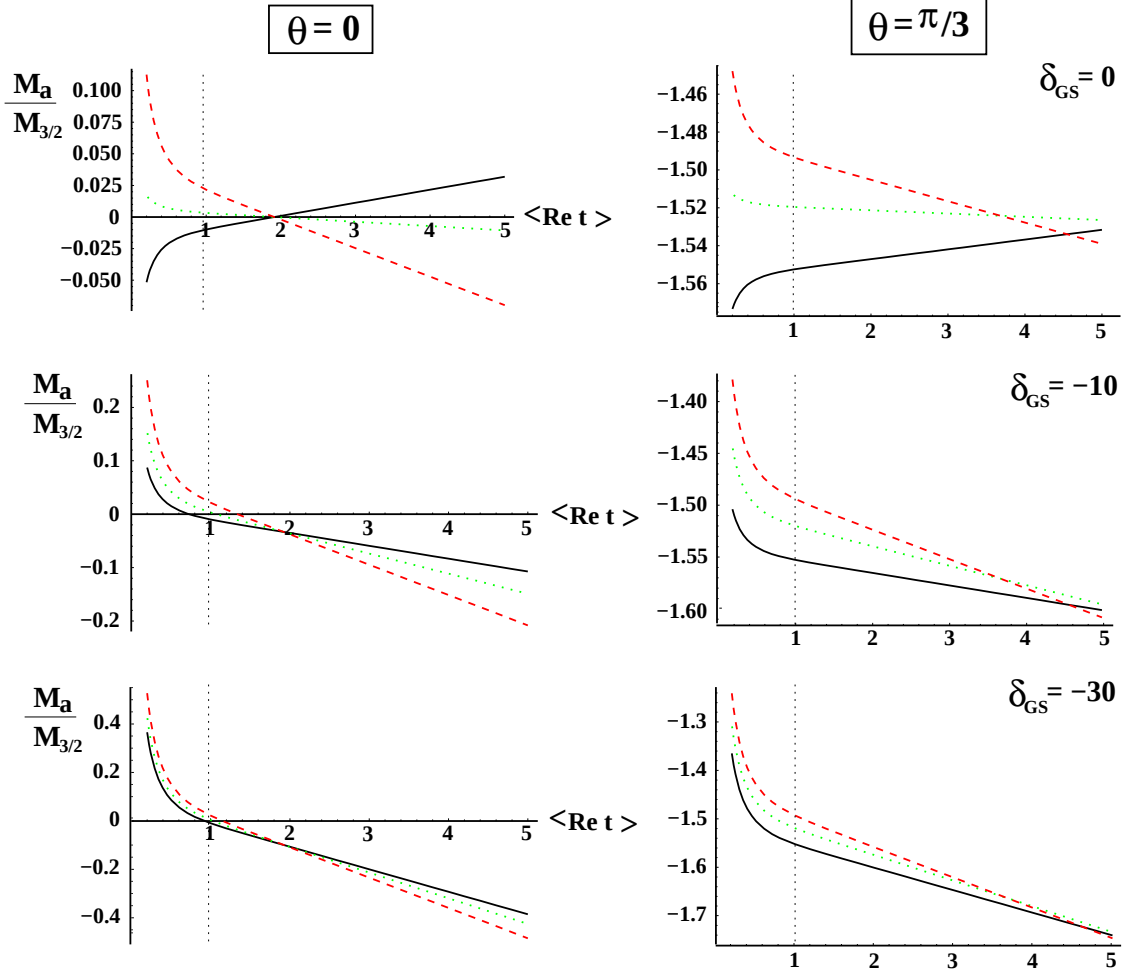
Figure 3: Relative Gaugino Masses vs. \langle \text{Re } t \rangle in the BIM O-II Model with \Lambda_{\text{UV}} = 2 \times 10^{16} \text{ GeV} . Relative sizes of the three gaugino masses M_1 (dashed), M_2 (dotted) and M_3 (solid) are displayed as a function of \langle \text{Re } t \rangle for two values of the Goldstino angle \theta and three representative values of \delta_{\text{GS}} . The vertical dotted line at \langle \text{Re } t \rangle = 1 indicates the moduli self-dual point where gaugino masses become independent of \delta_{\text{GS}} . When \sin \theta = 0 this point represents the case of leading anomaly contributions discussed in Section 3.1. All masses are relative to the gravitino mass m_{3/2} .
