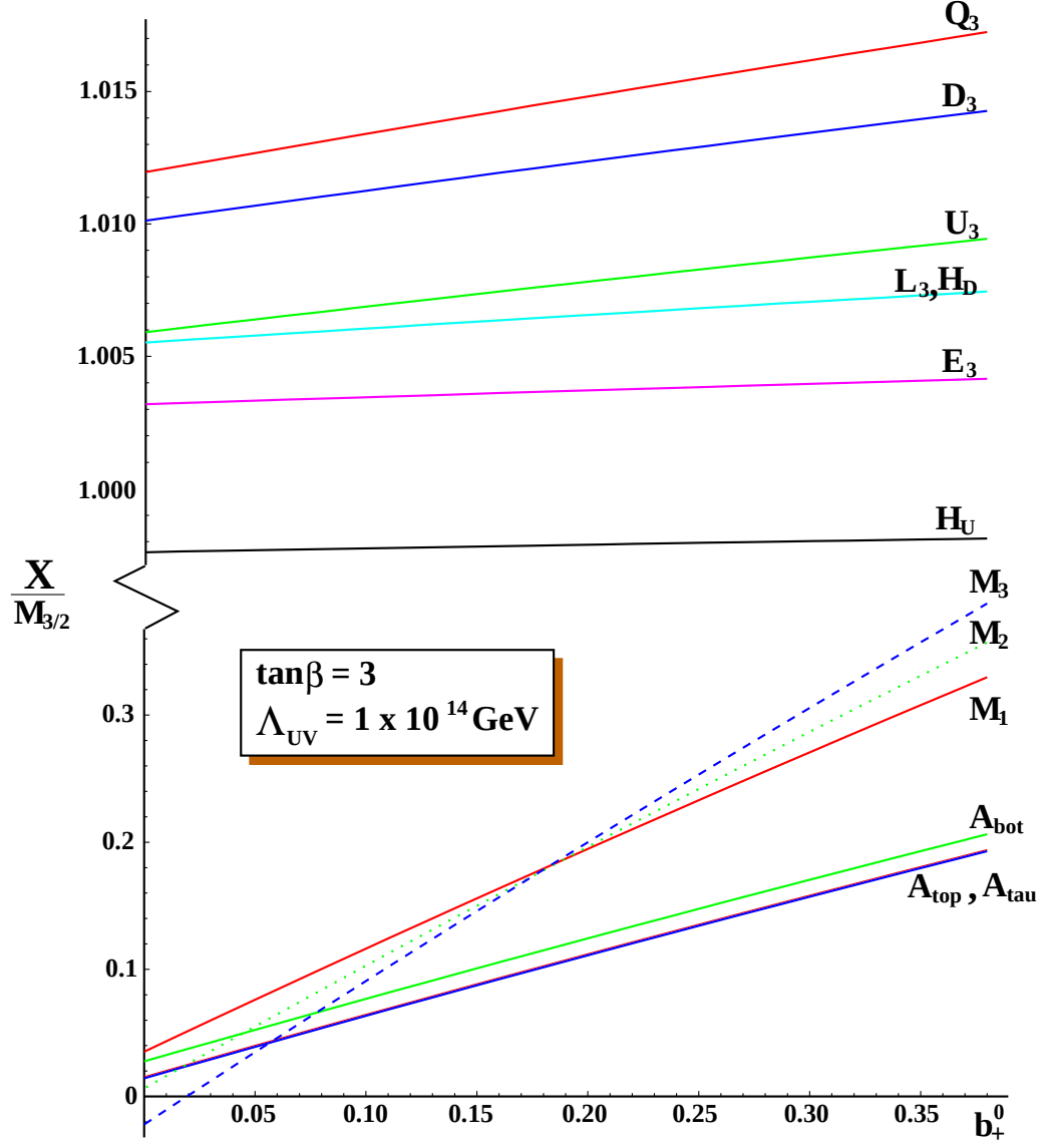
Figure 8: Spectrum of Soft Supersymmetry Breaking Terms in BGW Model. All values are given relative to the gravitino mass m_{3/2} at a scale \Lambda_{UV} = 1 \times 10^{14} \text{ GeV} as a function of the condensing group beta function coefficient b_+^0 .
