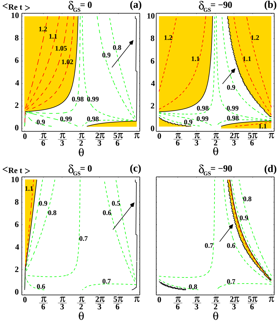
Figure 4: Ratio M_1/M_2 in BIM O-II Model. Contours of the absolute value of the ratio of U(1) to SU(2) gaugino masses are given for boundary scales of \Lambda_{\text{UV}} = 2 \times 10^{16} GeV for panels (a) and (b), and \Lambda_{\text{UV}} = 1 \times 10^{11} GeV for panels (c) and (d). The shaded area is the region of parameter space for which |M_1| \geq |M_2| . The arrow indicates the direction of smallest ratios as the discontinuity M_2 = 0 is approached. The contour M_1 = M_2 is given by the heavy solid line.
