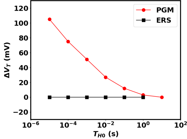
Figure 6.6: A demonstration of the device’s V_T shift; as the zero-bias hold time T_{H0} increases from 10 \mu s to 1 s, the PGM V_T (red) steadily decreases from 1.12 V to 1.02 V, while the ERS V_T (black) remains unchanged.
