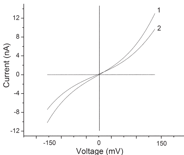
Figure 3. The reversal potentials measured for asymmetric solutions of different ionic composition in the presence of 4 μM Aβ oligomers added to one side. Trace 1, 100 mM KCl, cis; 100 mM CaCl 2 , trans. Trace 2, 100 mM KCl, cis; 50 mM CaCl 2 , trans. Bilayer composition was PC/PE (1/1, molar).
