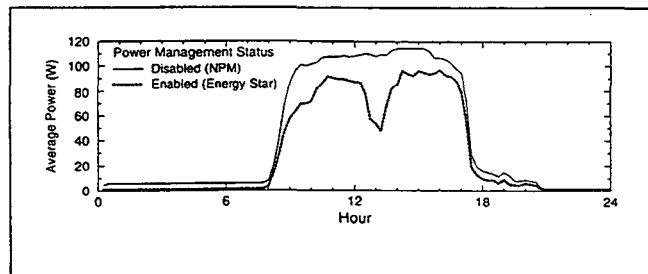
Figure 1. Hourly Average Energy Use with Power Management Enabled and Disabled; Weekday As-operated Energy Use: System S1, by Hour of Day
