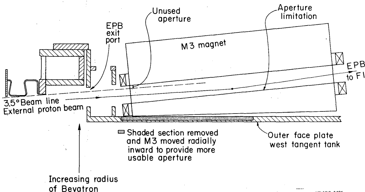
Fig. 2. External proton beam extraction magnet (M3) aperture restriction.
