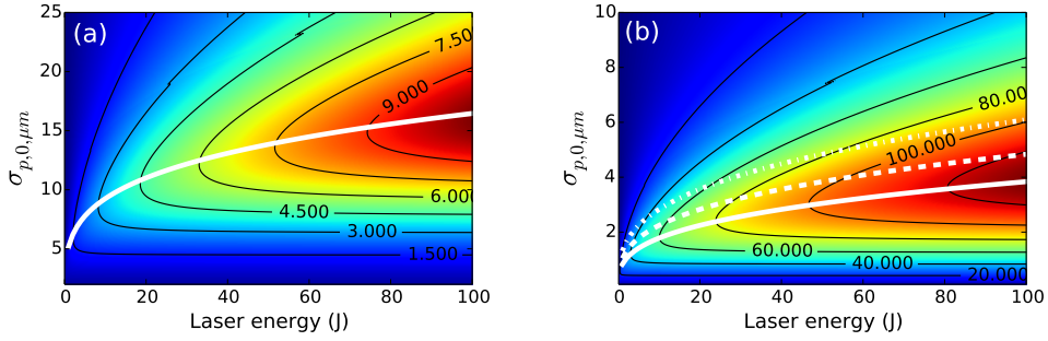
FIG. 12. (a): Total photon yield normalized to the number of electrons N_\gamma/N_e (color-coded image) as a function of both the laser pulse energy in Joules (horizontal axis) and laser pulse spot size \sigma_{p,0,\mu m} (left axis) for interaction in vacuum. Several isocontour lines are plotted in black color. Optimal transverse spot size \sigma_{p,opt,\mu m} as a function of laser pulse energy and given by eq. (46) is shown with thick white line. (b): Same as on (a) , but for the case of interaction in a waveguide. The optimal transverse spot size is in this case given by eq. (50) and is plotted with thick white line. Dashed and dot-dashed lines represent different fits to the optimum spot size and are explained in text.
