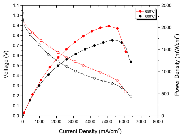
Figure 8. Sputtered cell (LSCF-YSZ/GDC/YSZ/Ni-YSZ) performance on hydrogen
