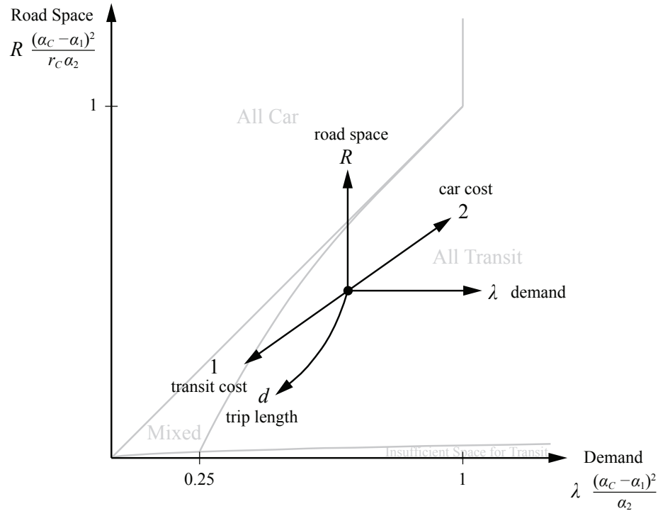
Figure 3.13. Effect of trip and mode parameters on a city's location on the scaled (\lambda, R) plane
