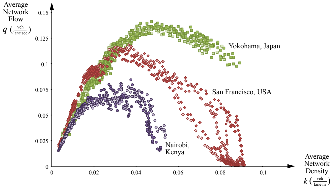
Figure 2.3. Experimental Macroscopic Fundamental Diagrams (MFDs) from measurement in Yokohama (Geroliminis & Daganzo, 2008) and simulations in San Francisco (Geroliminis & Daganzo, 2007) and Nairobi (Gonzales et al. , 2011)
