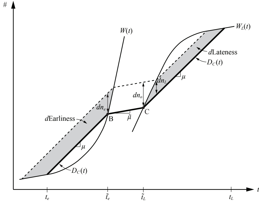
Figure 5.4. Decrease in earliness and increase in lateness resulting from a shift of B
