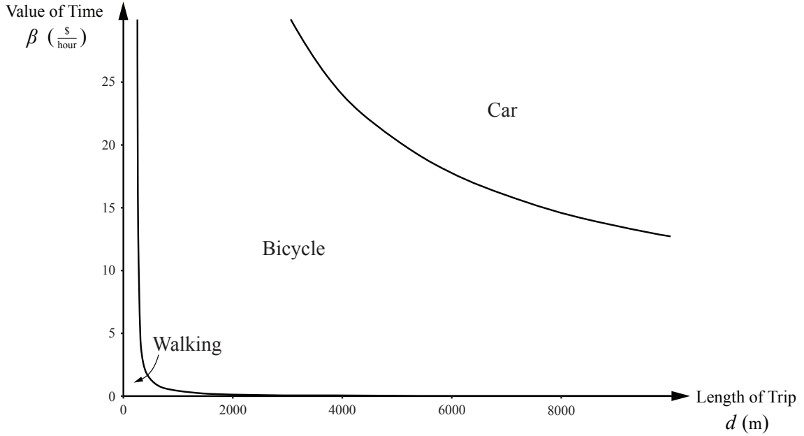
Figure 2.8. Comparison of individual modes over trip length and value of time showing which mode provides the minimum generalized cost per trip
