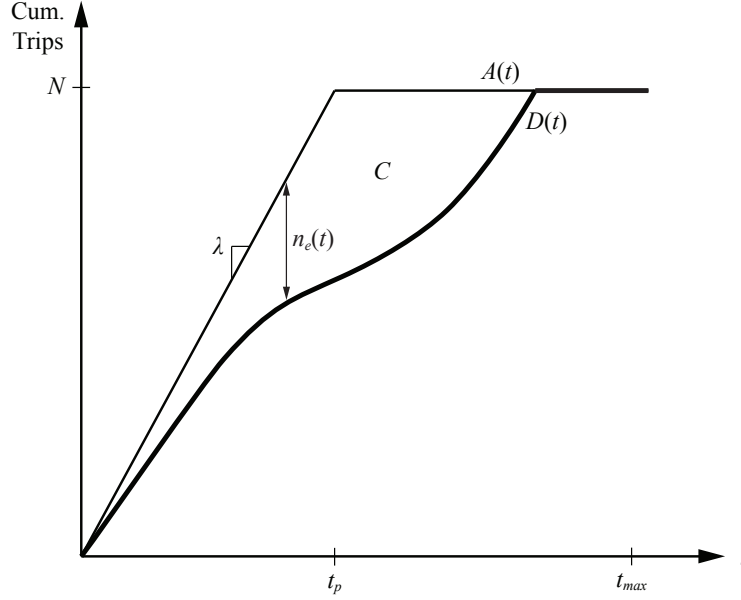
Figure 4.2. Queuing diagram for cars in a network in which exit flow declines with excess vehicle accumulation
