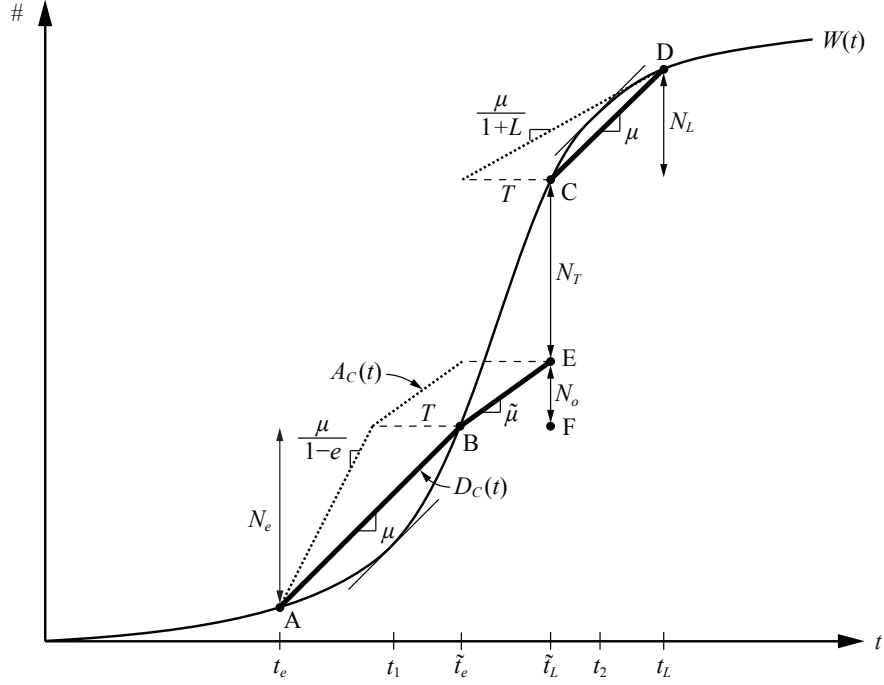
Figure 5.2. User Equilibrium for a bottleneck with a transit alternative
