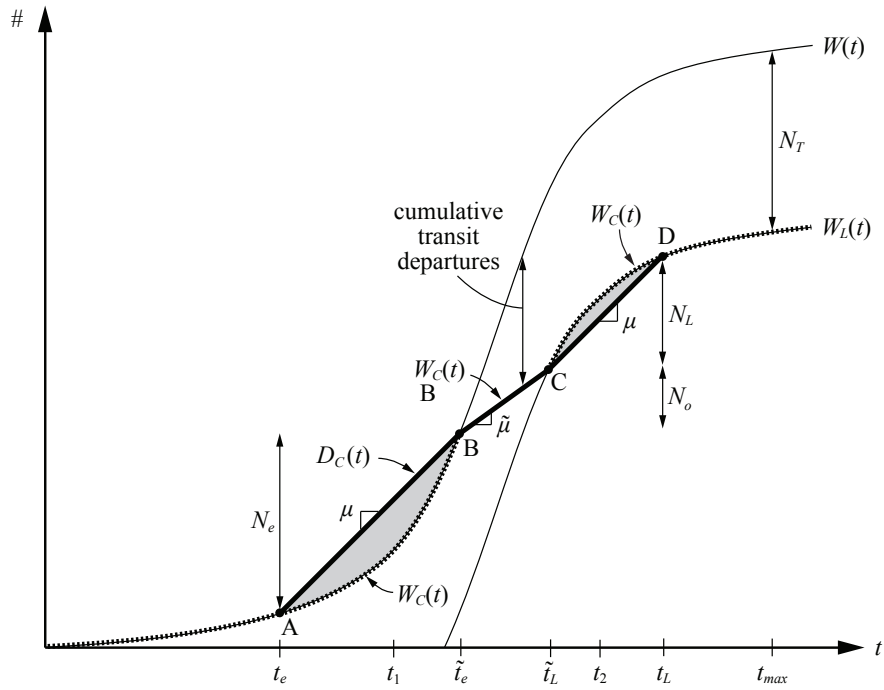
Figure 5.3. The departure curve for car that minimizes schedule delay given N_T
