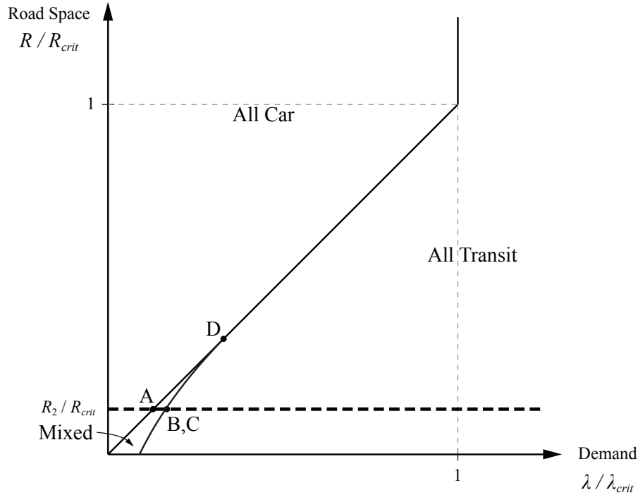
Figure 3.9. Summary of system optimum for all city structures with car and metro
