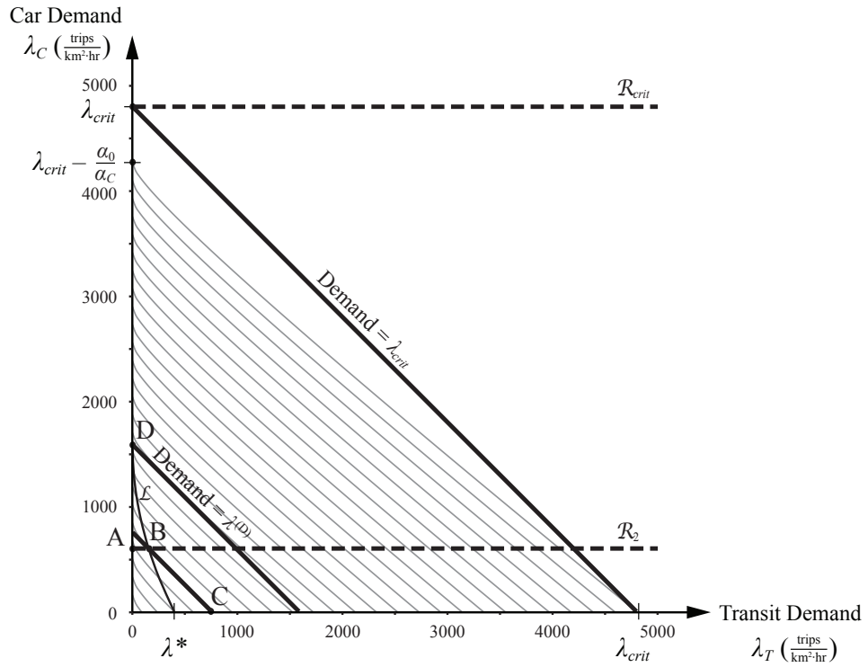
Figure 3.7. Cost contours and space constraints for a city with car and metro
