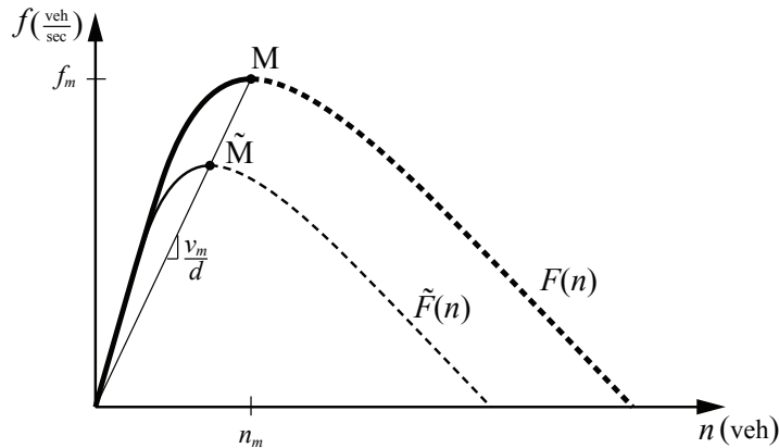
Figure 2.5. A generic concave Network Exit Function (NEF).
