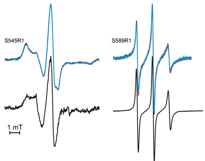
Fig. 3. Cw-EPR spectra of MTS spin label bound to positions 545 and 589 in the C-terminal domain of BetP in proteoliposomes. Top: In the absence (black) and presence of activating amounts of 400 mM NaCl (red) or 800 mM proline (blue) and 40 mM CrOx in the external buffer. Bottom: EPR spectra of the respective detergent solubilized BetP samples. Experimental parameters: modulation amplitude 1 G, time constant 100 ms, microwave power 1 mW, scan time 120 s, temperature stabilized at 20 °C. All spectra are normalized to the amplitude of the center resonance line.
