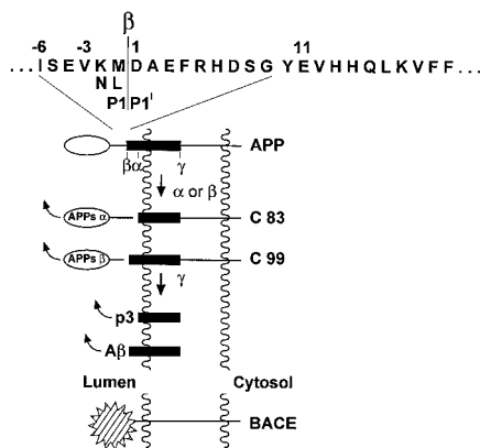
Fig. 1. Schematic structure of APP and BACE (not drawn to scale), showing proteolytic processing sites and cleavage products of APP. Wavy lines represent the cell membrane. The amino acid sequence of APP around the \beta -secretase cleavage site is numbered relative to the Asp1 start of A \beta . The position of the Swedish APP mutation, a substitution of P2: Lys \rightarrow Asn and P1: Met \rightarrow Leu, is indicated.
