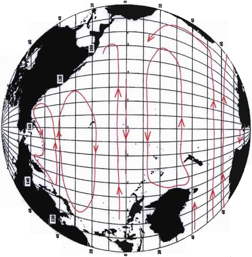
Fig. 2 Pacific Ocean circulation
