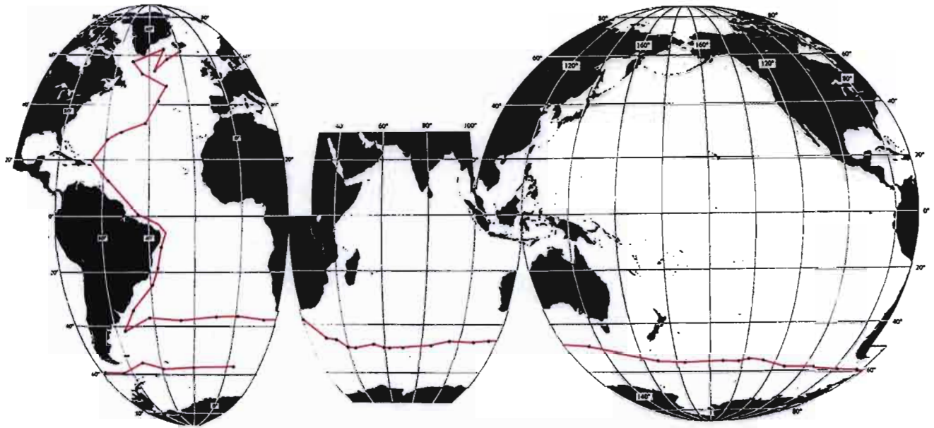
Fig. 29 Section from North Atlantic through Pacific
