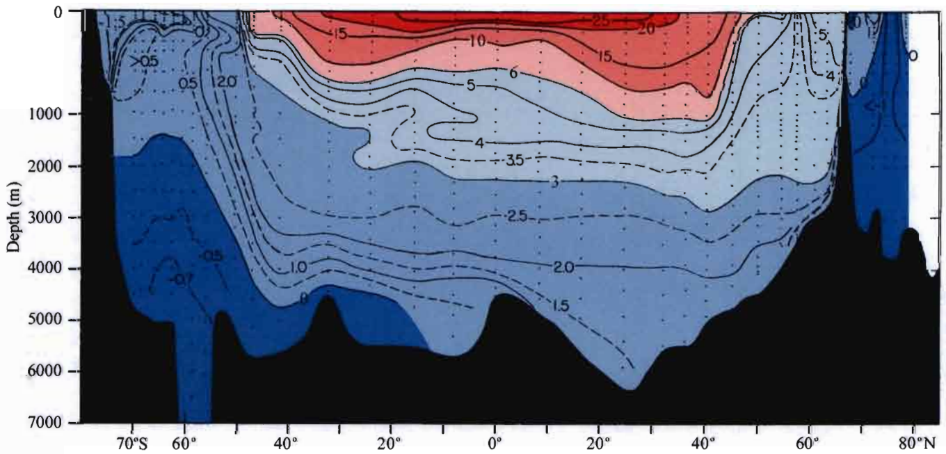
Fig. 23 Atlantic Ocean potential temperature along north-south section west of Mid-Atlantic Ridge
