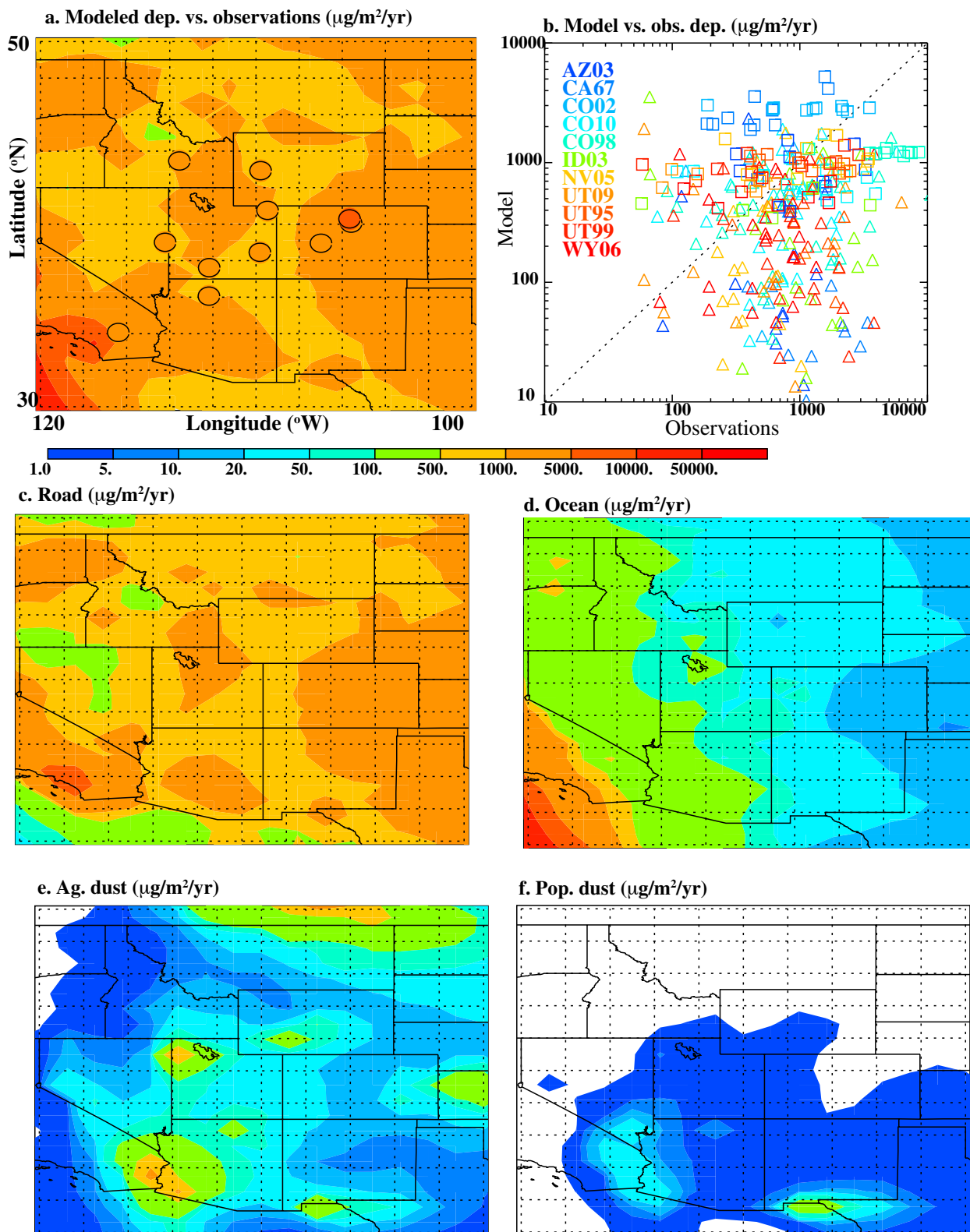
Fig. 3. Model estimates of microplastic deposition using the best estimate ( \mu\text{g}/\text{m}^2/\text{year} ). (A) Total plastic deposition from all the different model sources and the annual average of the observations at the sites (filled circles). (B) A scatterplot of the model versus observations for wet (triangles) and dry (squares) deposition ( r = 0.11 , n = 313 ). The station names are abbreviated from the National Atmospheric Deposition Network, following SI Appendix, Table S1 , and the latitude and longitude are as follows: AZ03 (36.1°N, 247.8°E), CA67 (34.1°N, 243.6°E), CO02 (40.1°N, 254.4°E), CO10 (39.0°N, 253.0°E), CO98 (40.3°N, 254.4°E), ID03 (43.5°N, 246.5°E), NV05 (39.0°N, 245.8°E), UT09 (38.46°N, 250.2°E), UT95 (40.8°N, 250.5°E), UT99 (37.6°N, 247.8°E), and WY06 (42.9°N, 250.2°E). The total microplastic deposition (A) is the sum of the road tire and braking (C), ocean (D), agricultural dust (E), and population dust (F), which is the dust generated downstream from population centers. Notice that the population source is not plotted as it is zero in the best estimate.
