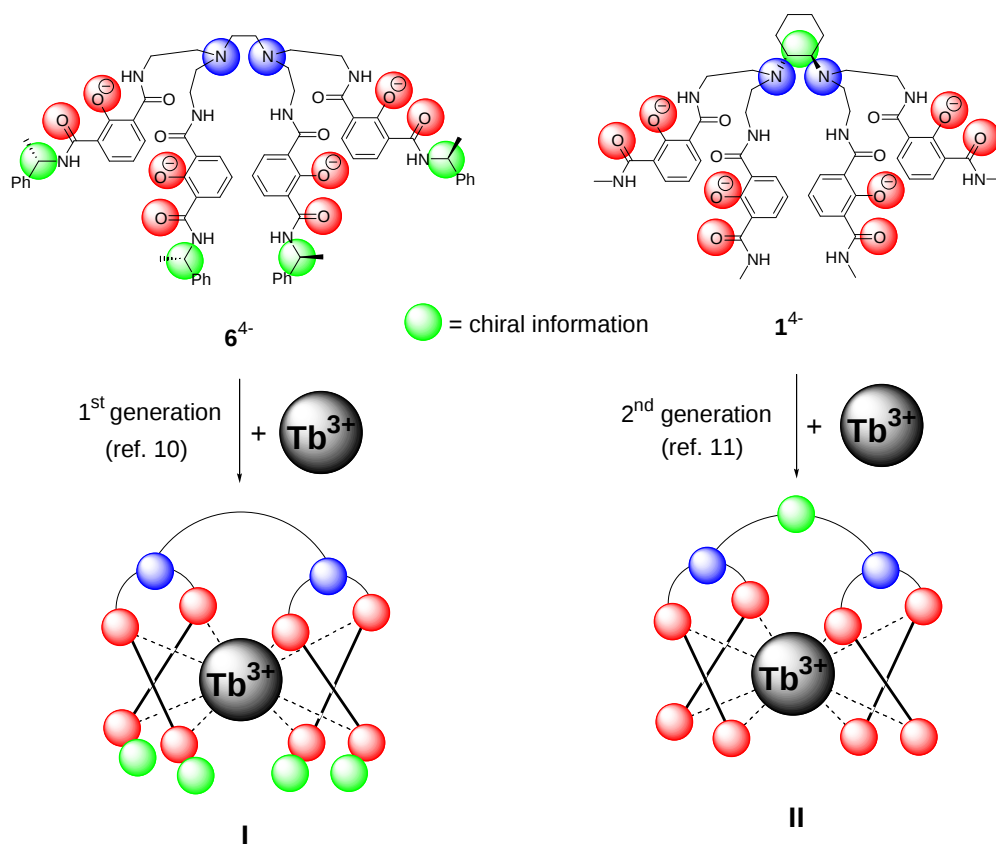
Figure 3. Schematic representation of the design change for the 1 st to the 2 nd generation of enantiopure, octadentate ligands: Chiral information (green spheres) in the polyamine backbone for II (blue part) instead of incorporation into the chelating IAM moiety in I (red part).
