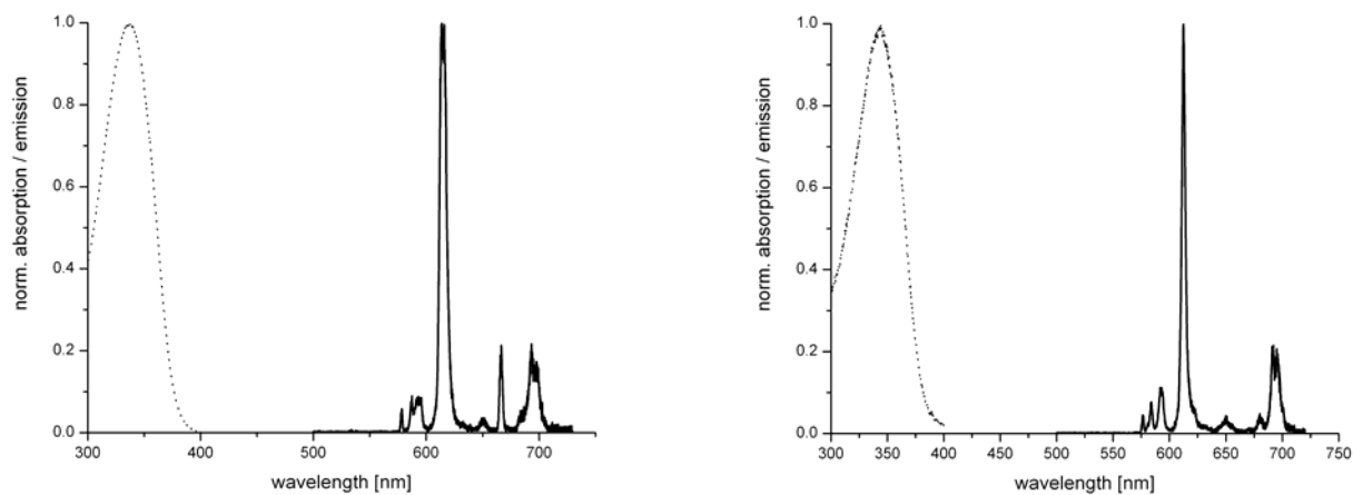
Figure 7. Normalized absorption (dotted lines) and steady-state emission (solid lines) of [Eu(H3)(H 2 O)] (left, \lambda_{\text{exc}} = 328 nm) and [Eu(H4)(H 2 O)] (right, \lambda_{\text{exc}} = 340 nm) in 0.1 M aqueous Tris buffer at pH 7.4.
