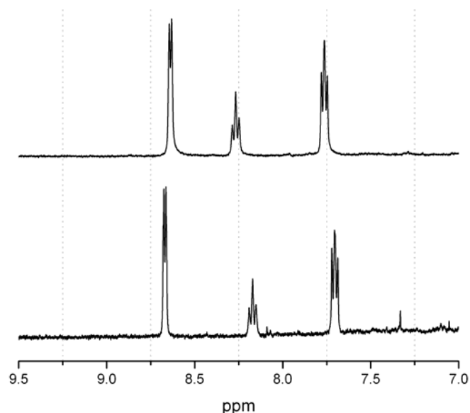
Figure 5. Aromatic region of the ^1\text{H} NMR spectra (500 MHz) of saturated solutions of [\text{Eu}(\text{H}3)(\text{H}_2\text{O})] (top) and [\text{Eu}(\text{H}4)(\text{H}_2\text{O})] (bottom) 11 in \text{CD}_3\text{OD} .
