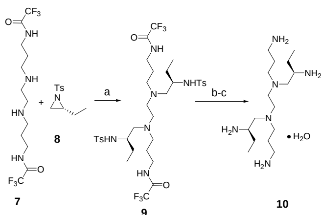
Scheme 1. Synthesis of the enantiopure, tetrapodal hexamine backbone 10 .
