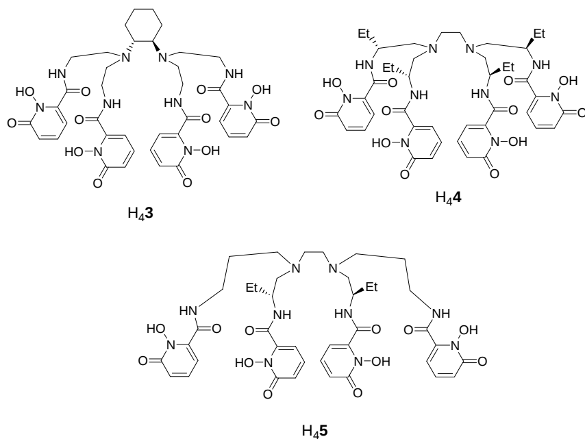
Figure 2. Ligands based on 1-hydroxy-2-pyridinone (1,2-HOPO).
