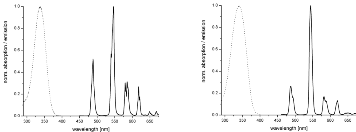
Figure 6. Normalized absorption (dotted lines) and steady-state emission (solid lines) of [Tb(H1)] (left, \lambda_{\text{exc}} = 340 nm) and [Tb(H2)(H 2 O)] (right, \lambda_{\text{exc}} = 340 nm) in 0.1 M aqueous Tris buffer at pH 7.4.
