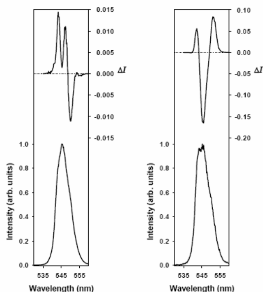
Figure 9. CPL (top) and total luminescence (bottom) spectra of the ^5D_4 \rightarrow ^7F_5 transition of [Tb(H 2 )(H 2 O)] in MeOH (left: c \approx 1 mM, excitation at \lambda = 360 nm) and in 0.1 M Tris buffer at pH 7.4 (right: saturated solution, excitation at \lambda = 346 nm).
