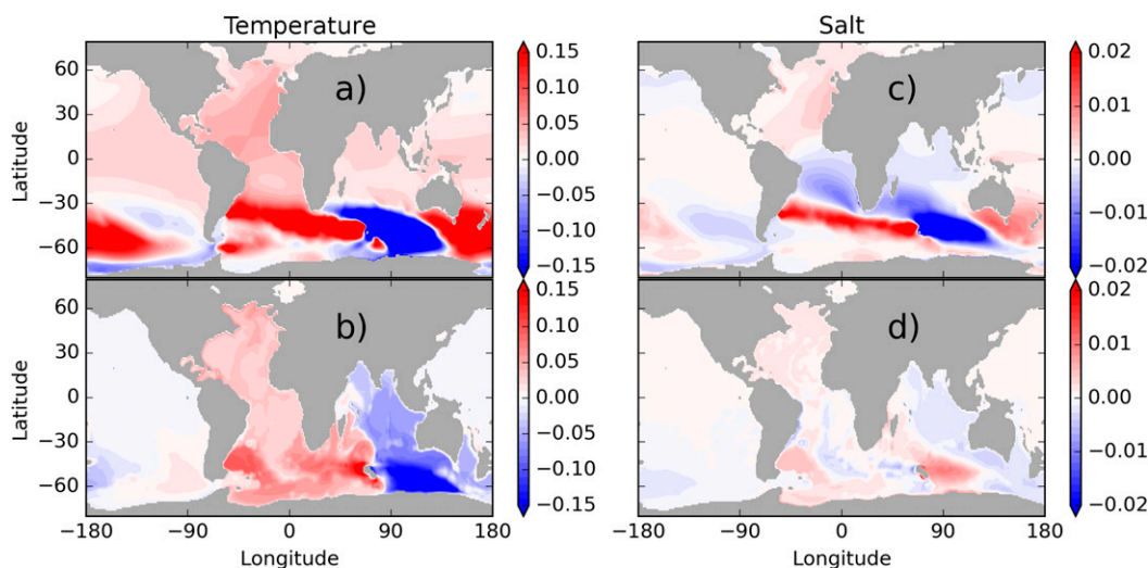
FIG. 6. The (a),(b) temperature (°C) and (c),(d) salinity (psu) differences between CTRL and noKP (noKP – CTRL) for the (top) upper (0–1000 m) and (bottom) deep ocean average below 1000 m.
