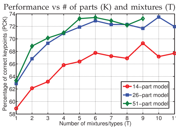
Fig. 7. We show the effect of model structure on pose estimation by evaluating PCK performance on the Parse dataset. Overall, increasing the number of parts from 14 to 26 (by instantiating parts at limb midpoints in addition to joints) improves performance. Instantiating additional middle parts between limb midpoints and joints (from 26 to 51) yields no clear improvement. In all cases, increasing the number of mixtures improves performance, likely due to the fact that more orientations and foreshortening can be modeled. We find that a 26-part model with six mixtures provides a good tradeoff of performance versus computation.
